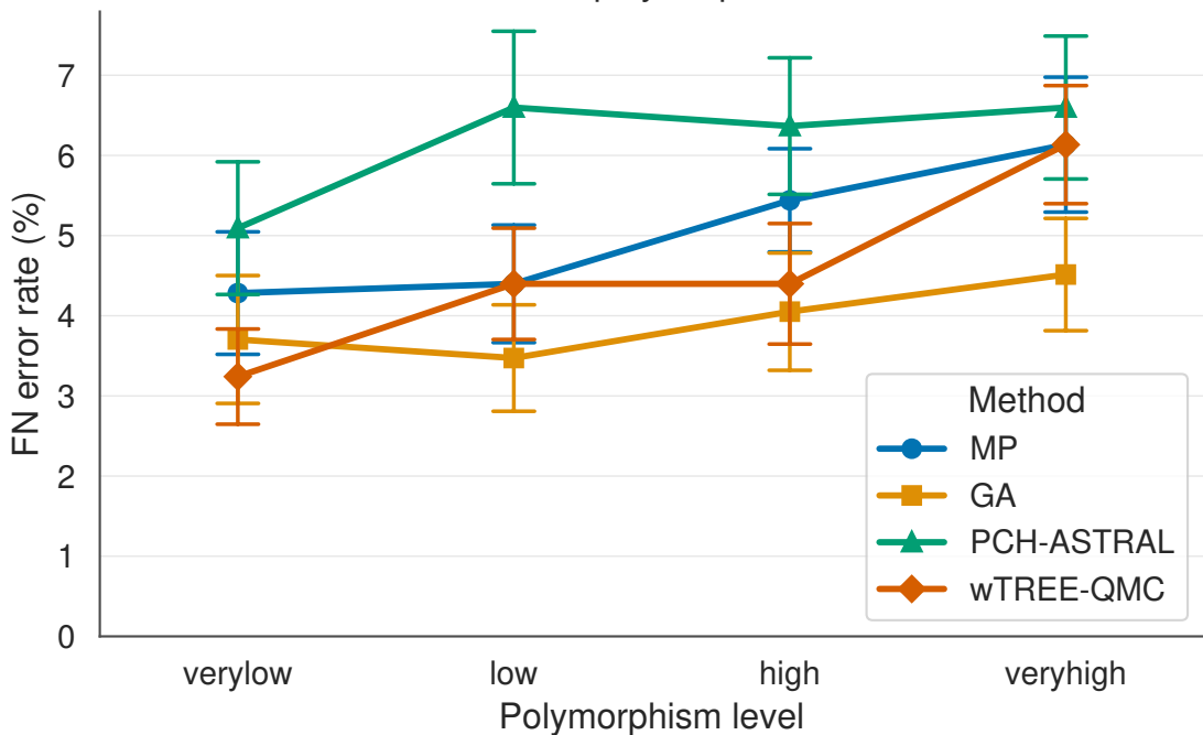
FN error vs polymorphism level
