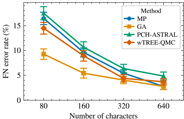
FN error vs number of characters
