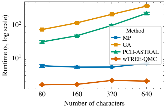
Runtime vs number of characters
