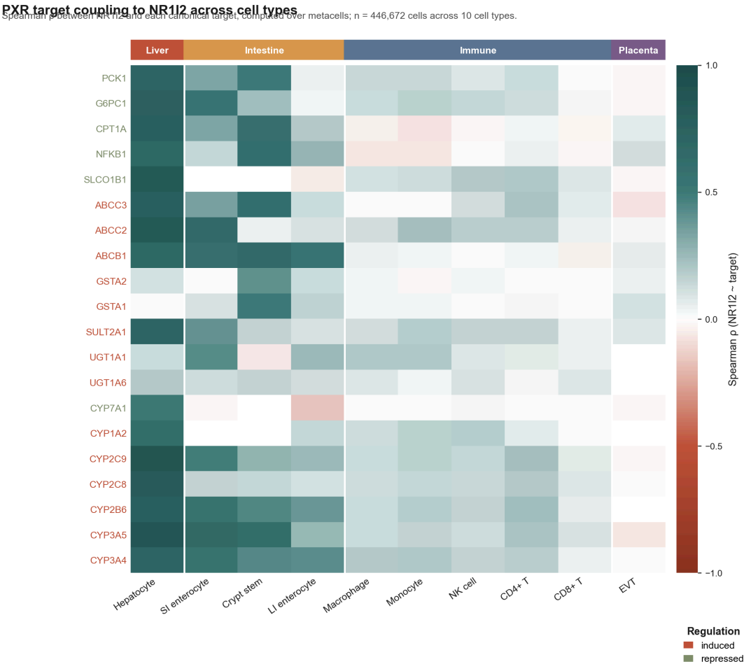
Main coupling heatmap across the 10 cell types
