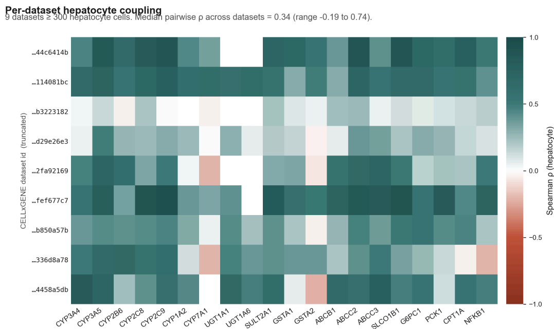
Per-dataset hepatocyte coupling
