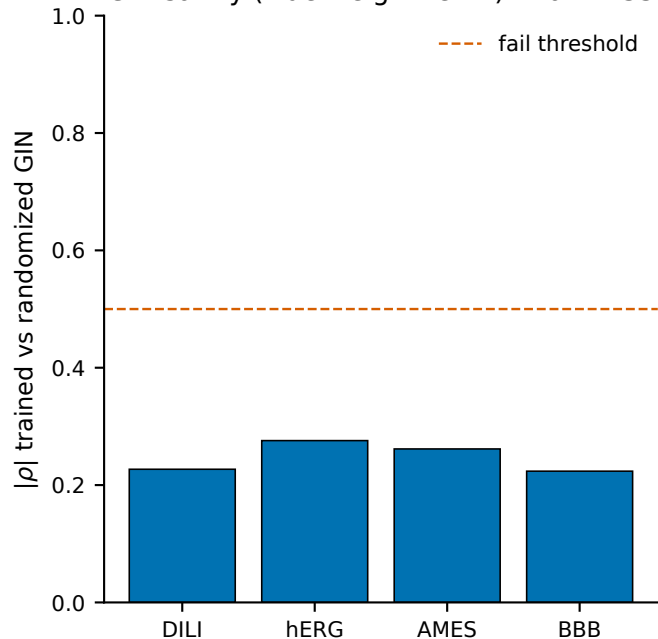
GIN sanity (true weight reinit) — all PASS
