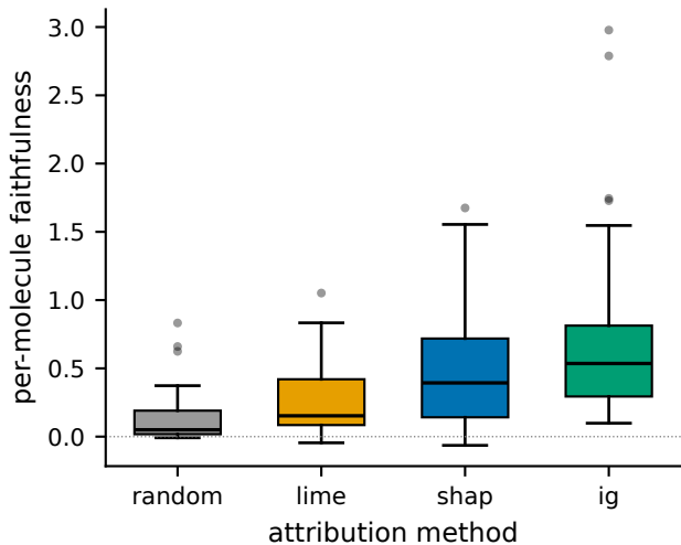
Paper 1 · Faithfulness by method (all cells)
