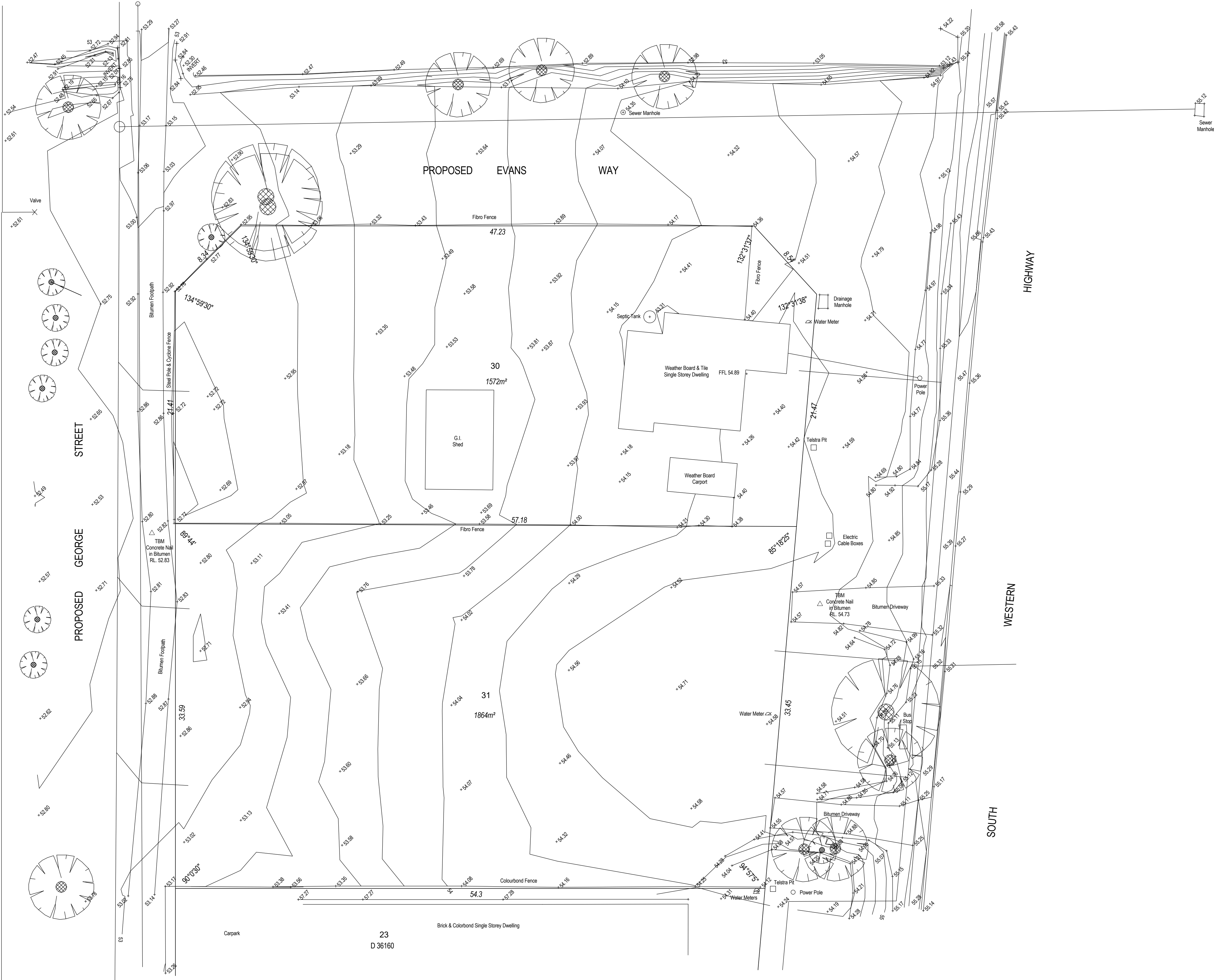
1 Feature Survey 1 : 200
