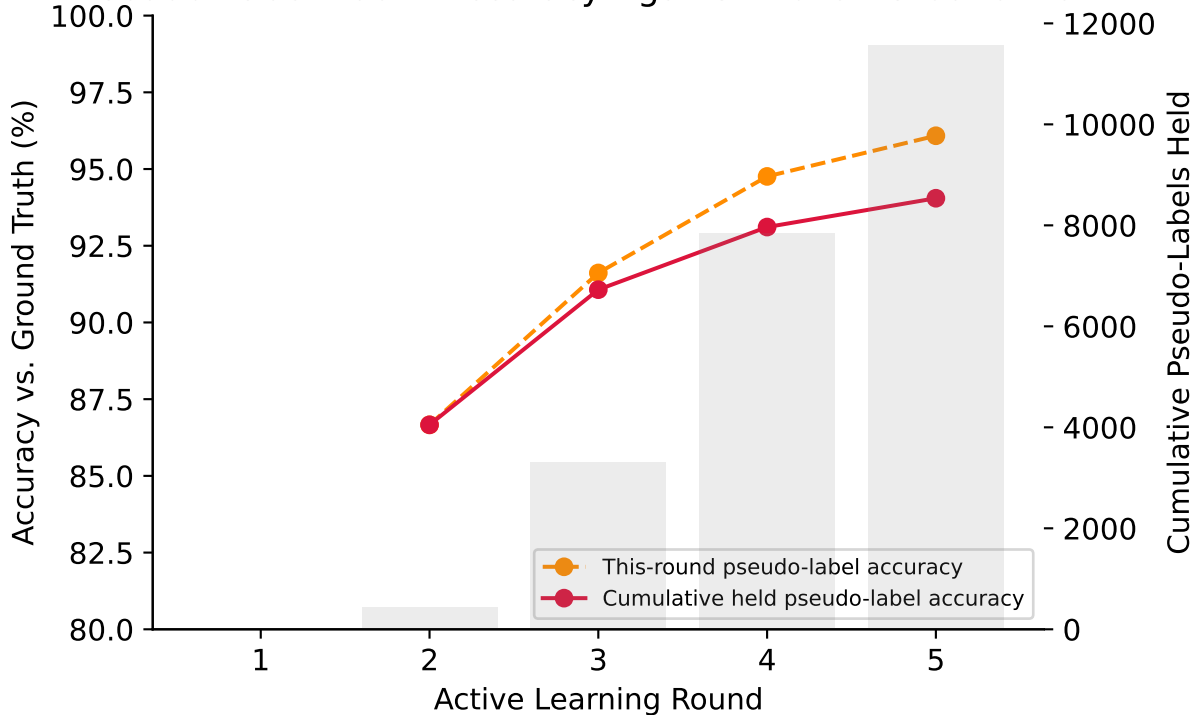
Pseudo-Label Audit: Accuracy Against Frozen Ground Truth
