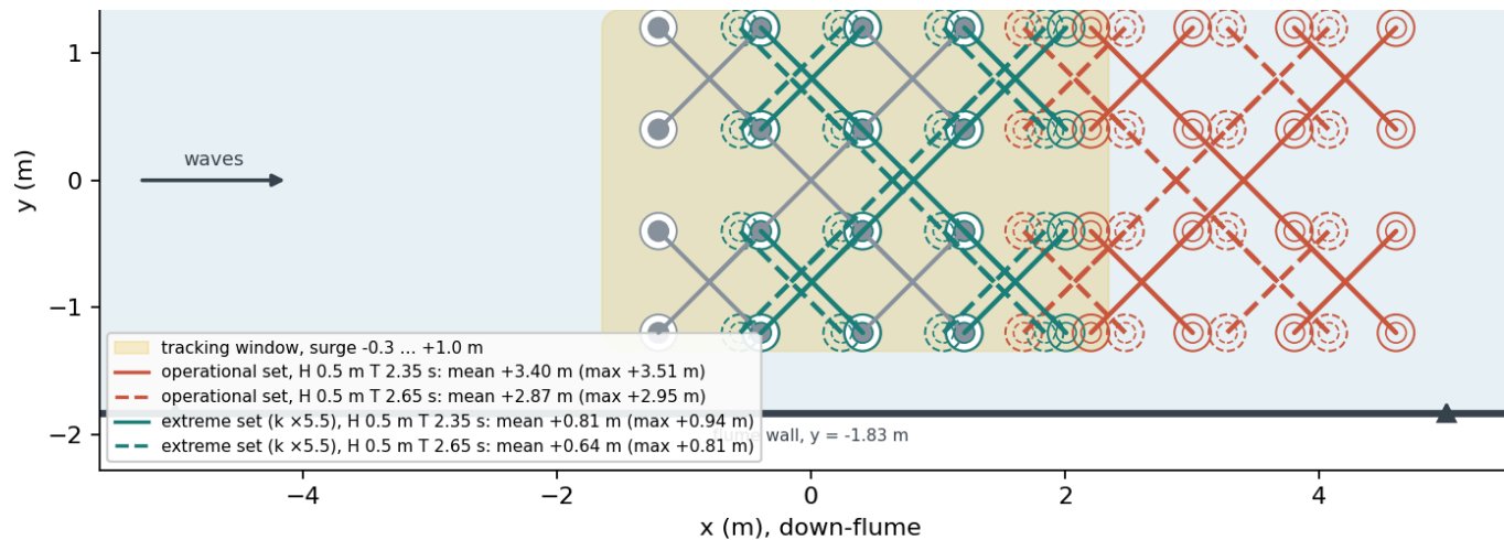
H = 0.5 m mean positions of both cord sets against the tracking window (FloatSim, drift sum)
