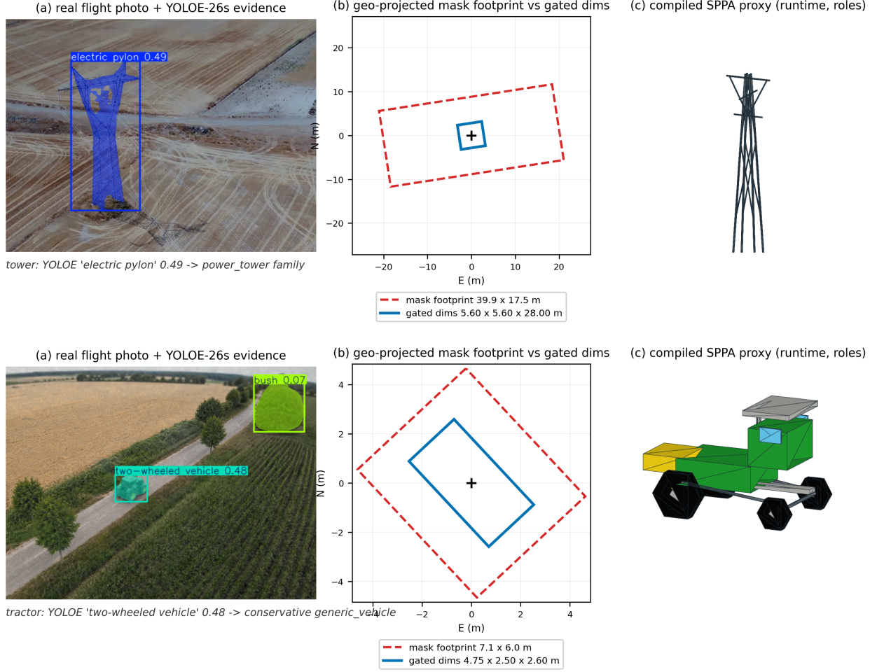
Figure 11: Real flight-photo probes end to end (exploratory, no 3D ground truth; declared assumed-flight telemetry). Rows: tower and tractor photos recorded for this paper. (a) YOLOE-26s evidence (bbox, native mask, confidence). (b) Geo-projected mask footprint (dashed red) against the gated metric dims (blue): the tower’s 39.9 \times 17.5 m footprint is clamped to 5.60 \times 5.60 \times 28.00 m by the family aspect prior; the tractor’s 7.1 \times 6.0 m is fused to 4.75 \times 2.50 \times 2.60 m. (c) The compiled runtime proxies (396 and 576 triangles): the detector mislabels the tractor as two-wheeled vehicle , which exercises the conservative generic_vehicle routing instead of a committed wrong token.
