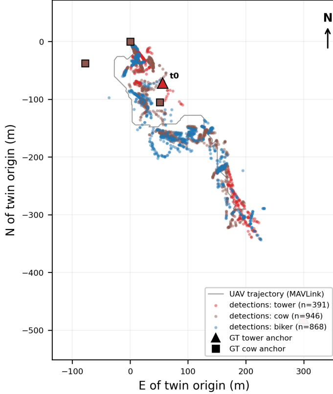
Recorded flight over the georeferenced Ejea twin (2026-06-20)
