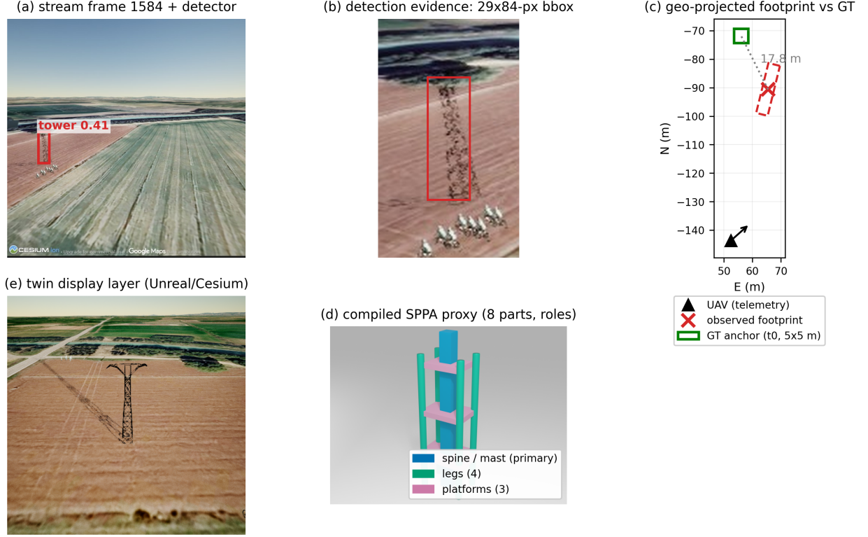
Figure 4: Worked end-to-end example on measured field data (frame 1584 of the real stream, Section 4.10). (a) The detector reports a tower at confidence 0.41, the only hypothesis in this frame. (b) Detection evidence: the 29 \times 84 -px detector bbox, cropped and magnified. (c) The geo-projected footprint ( 18.0 \times 4.2 m observed) against the exact simulator anchor of tower t_0 ; the localization gap is set by the monocular observation geometry and is quantified for the whole stream in RP. (d) The compiled eight-part lattice_tower proxy with semantic roles (spine, legs, platforms), placed directly below the real crop for silhouette comparison. (e) The Unreal/Cesium twin layer in which the emitted actor is displayed.
