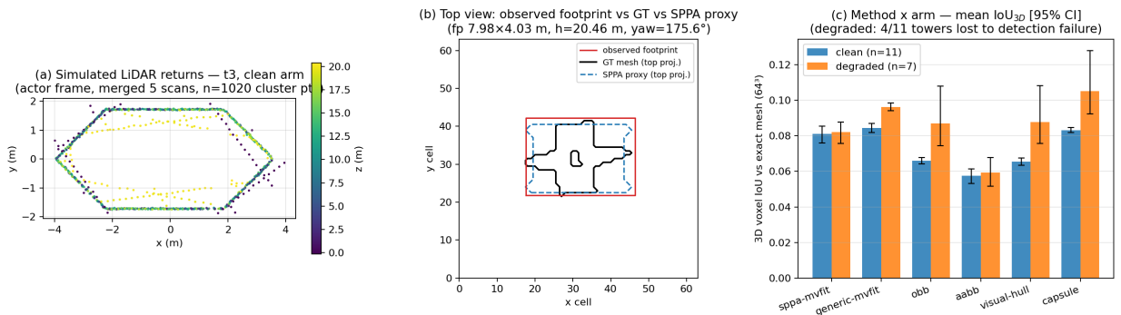
Figure 14: E14 simulated-LiDAR demonstration (exploratory post-hoc; returns are UE raycasts, not hardware). (a) Simulated LiDAR-class returns on tower t3. (b) Recovered footprint and SPPA proxy against the ground-truth top silhouette: the camera-less contract recovers the envelope (footprint, yaw, height) reliably. (c) Voxel-exact 3D IoU by arm and method: all methods sit at the lattice’s sub-voxel structural ceiling ( \approx 0.08 ); SPPA’s advantage in this setting is proxy economy, not IoU leadership.
