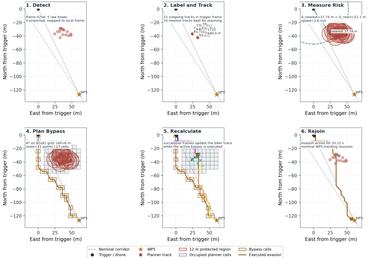
Figure 5: Six-stage reconstruction of the audited PORCE maneuver, from YOLO detection to nominal-route rejoin. All panels use the same local ENU view centered on the trigger state, while successive panels add the projected detections, planner subset, reaction horizon, discretized bypass, executed evasion, and final rejoin.
