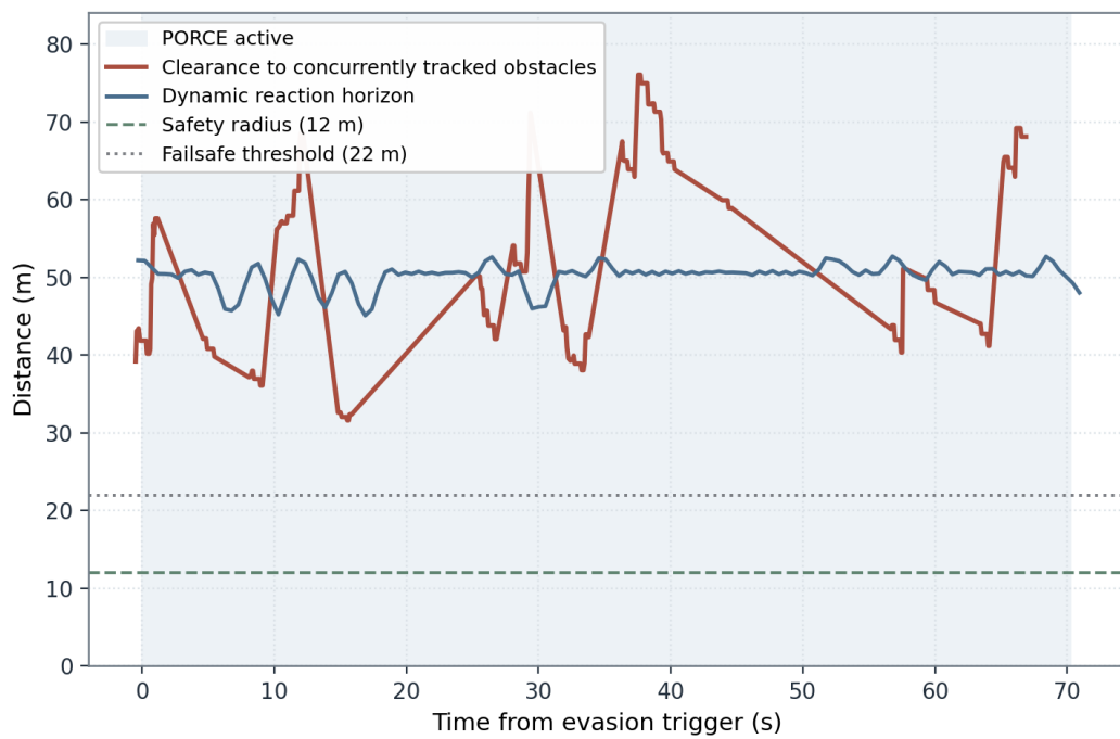
Figure 8: Clearance and reaction-distance time series for the audited maneuver. The time-synchronized clearance to concurrently tracked obstacles remains above both the configured 12.00 m hard safety radius and the 22.00 m failsafe threshold while the local evasion route is active.
