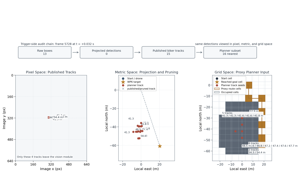
Figure 6: Perception-to-planner audit chain for the trigger-side biker event. The same detections are displayed as camera boxes, local metric points, and inflated planner-grid cells.
