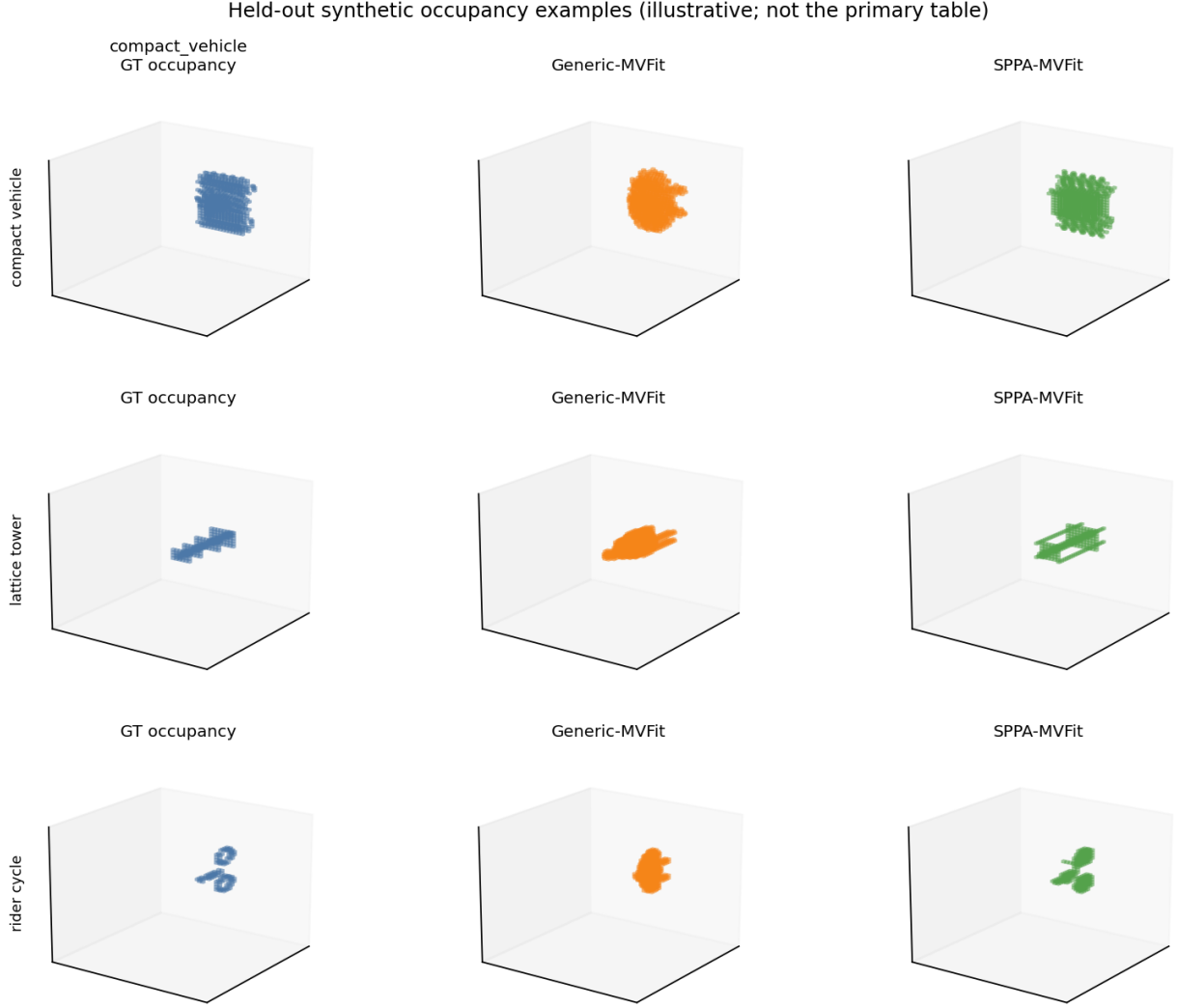
Figure 2: Held-out synthetic occupancy examples for three families: ground truth (left), Generic-MVFit (center), and SPPA-MVFit (right). Illustrative only; the confirmatory decision uses Table 2, not this figure.
