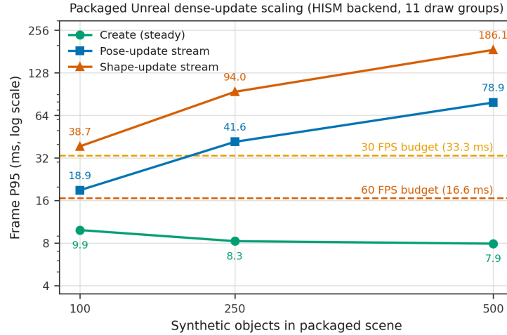
Figure S5: Packaged-runtime scaling (HISM backend, dense-update streams), moved from the main text: frame P95 versus object count for the create, pose-update, and shape-update streams. The 33.3 ms line marks a desktop 30 FPS budget; dense shape updates exceed it already at 100 objects and dense pose updates between 100 and 250, while the sparse 10% changed-track schedule of the condensed runtime table in the main text stays below it at 500 objects. Run note: the plotted series comes from the original scaling run 20260703T033655Z (CSV logging active; 100-object shape frame P95 38.7 ms), whereas the condensed runtime table in the main text and the table above quote the isolated no-CSV rerun 20260703T033840Z (37.126 ms). The two runs differ only in absolute milliseconds; dense shape updates exceed the 33.3 ms budget from 100 objects in both, so the conclusion is unchanged.
