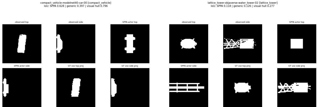
Figure S7: External sanity check, qualitative (moved from the main text). Left: a ModelNet40 car where the family graph helps (SPPA 0.628 vs generic 0.397). Right: an Objaverse water tower whose horizontal tank mismatches the vertical tower template (SPPA 0.118 vs generic 0.126)—the template–instance mismatch failure mode. Panels show observed masks, SPPA actor projections, and ground-truth voxel projections.
