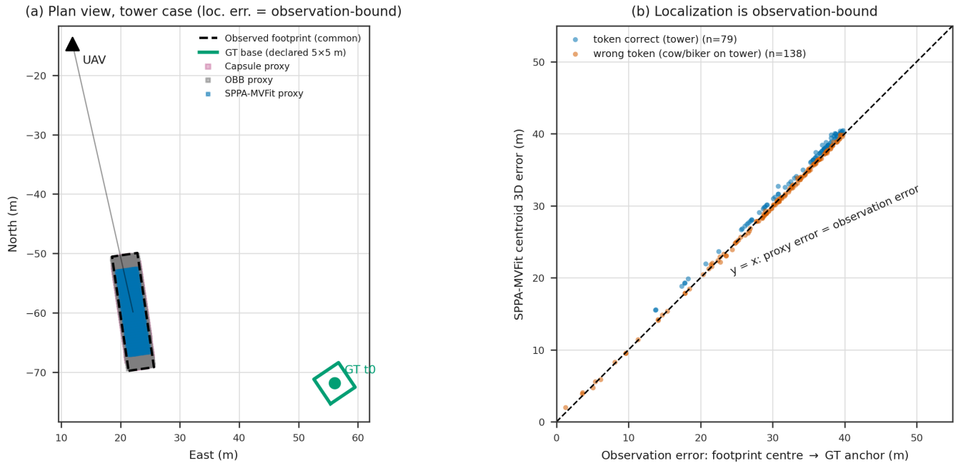
Figure S8: Real-stream localization panels (moved from the main text). (a) Plan view of a tower case: the observed footprint (dashed) and all fitted proxies sit \approx 35 m from the exact anchor—observation-bound. (b) Fitted-centroid error versus observation error: the identity line holds for all methods.
