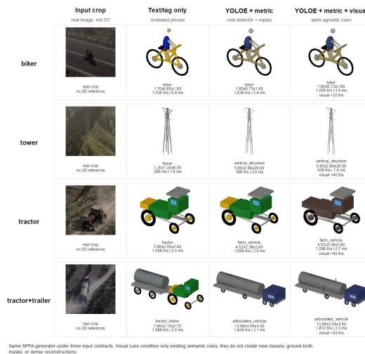
Figure S4: SPPA input-mode ablation on the four real-image probes: text-only, YOLOE+metric, and YOLOE+metric+visual contracts through the same deterministic generator. An ablation of SPPA evidence handling, not ground-truth 3D evaluation.
