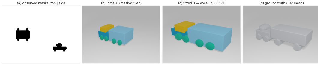
Figure S6: Fitting of SPPA-MVFit on a held-out actor (moved from the main text): (a) the observed silhouette pair, (b) initialization from the observed mask extents, (c) the converged eight-part proxy, and (d) the ground-truth voxel mesh.
