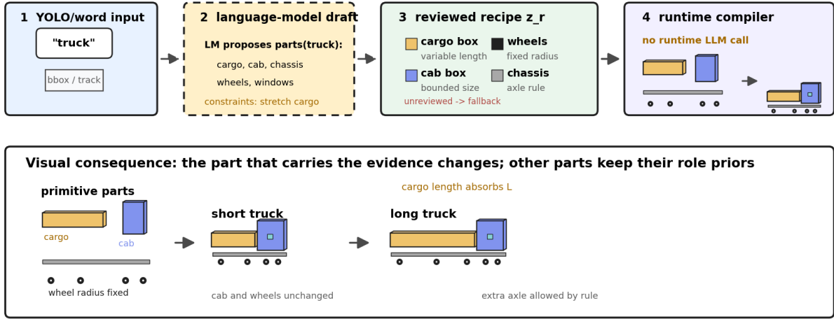
Figure S1: SPPA semantic-label-to-parts-to-3D mechanism for the truck archetype (moved from the main text). A language model, ontology tool, or human author may draft candidate part roles offline, but runtime execution uses only a reviewed versioned recipe z_r . An input label activates an offline draft, the draft is reduced to reviewed part roles and bounded update rules, and runtime compiles those roles into primitive geometry. The short and long proxy variants illustrate the implemented role-specific rule: cargo length changes while cab and wheel priors remain bounded, so the object is not represented by root-scaling a single box.
