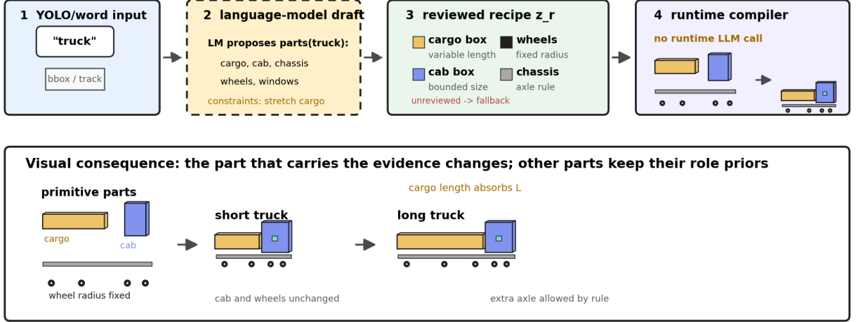
Figure 3: SPPA semantic-label-to-parts-to-3D mechanism for the truck archetype. A language model, ontology tool, or human author may draft candidate part roles offline, but runtime execution uses only a reviewed versioned recipe z_r : an input label or word activates an offline draft, the draft is reduced to reviewed part roles and bounded update rules, and runtime compiles those roles into primitive geometry. The short and long proxy variants illustrate the implemented role-specific rule: cargo length changes while cab and wheel priors remain bounded, so the object is not represented by root-scaling a single box.
