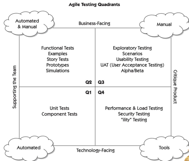
Figure 6-1 Agile Testing Quadrants
