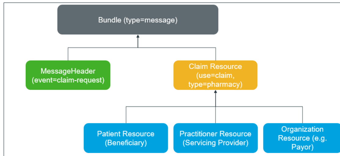
Figure 1: FHIR Bundle Resource Hierarchical Structure
