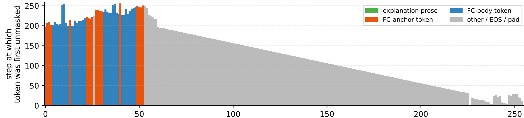
Diffusion denoising trajectory · remasking = entropy · final FC blocks = 2 · explanation tokens = 0 · FC tokens = 52
