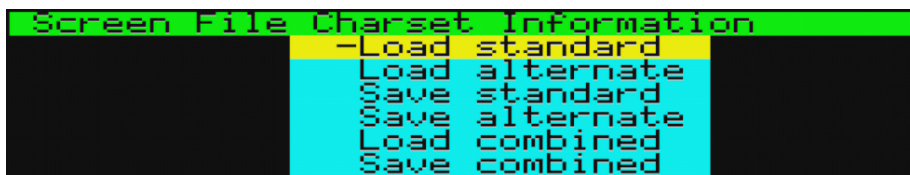
Figure 11: Charset menu
