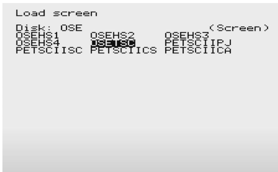
Figure 9: Load screen
