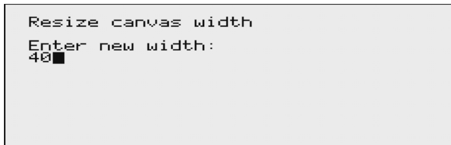
Figure 5: Resize width
