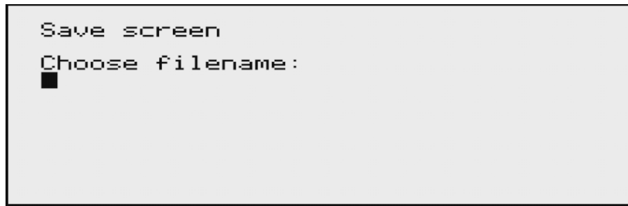
Figure 8: Save screen
