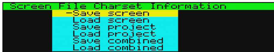
Figure 7: File menu
