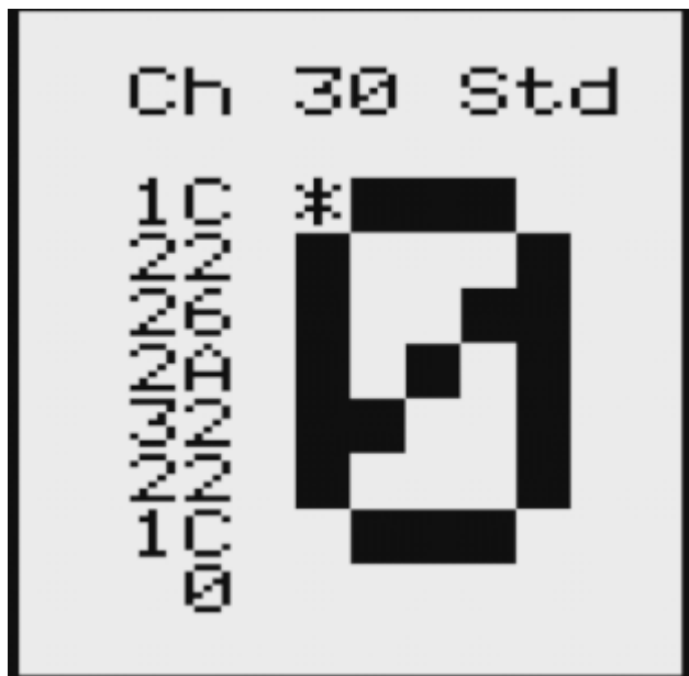
Figure 14: Character editor
