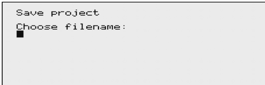
Figure 10: Save project
