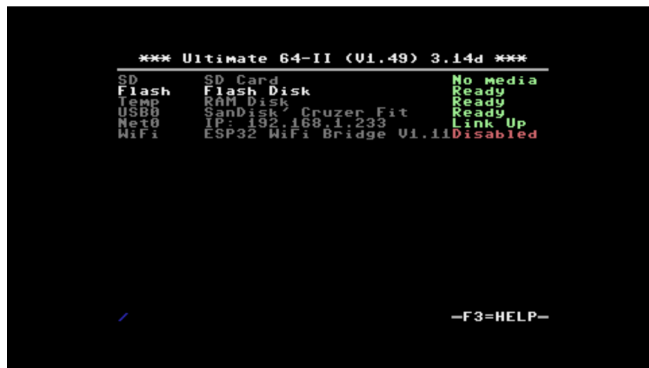
Figure 5: Ultimate UI
