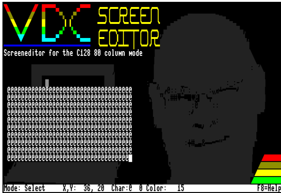
Figure 29: Select mode
