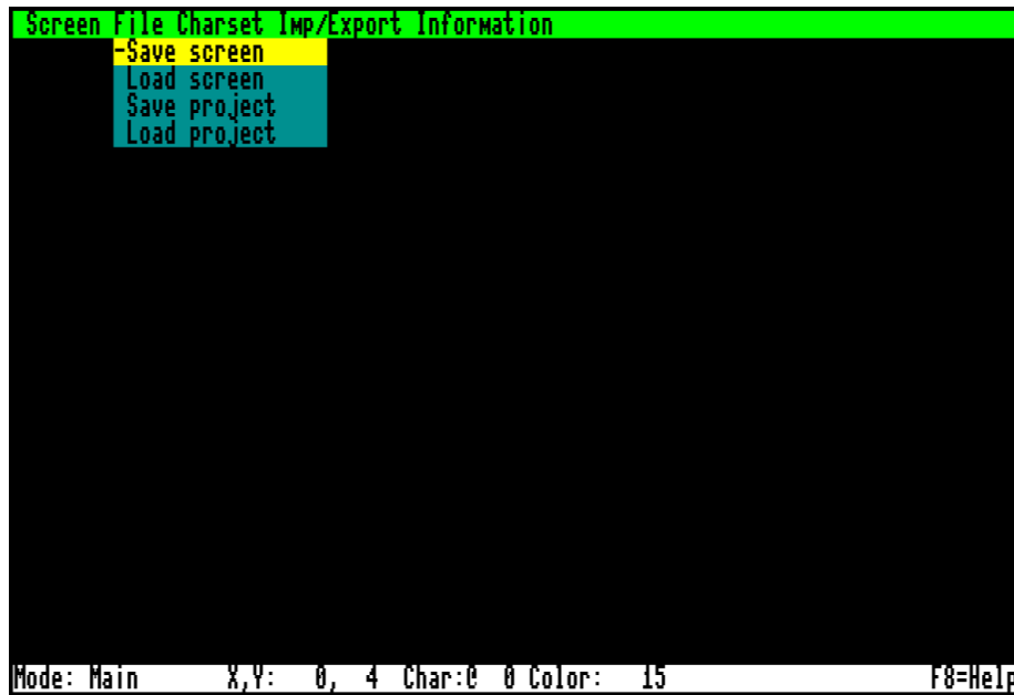
Figure 11: File menu
