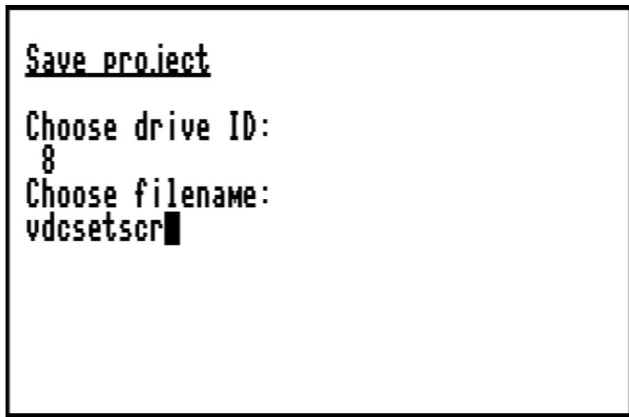
Figure 16: Save project
