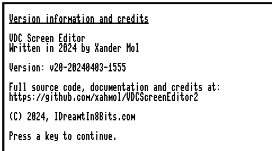
Figure 24: Information
