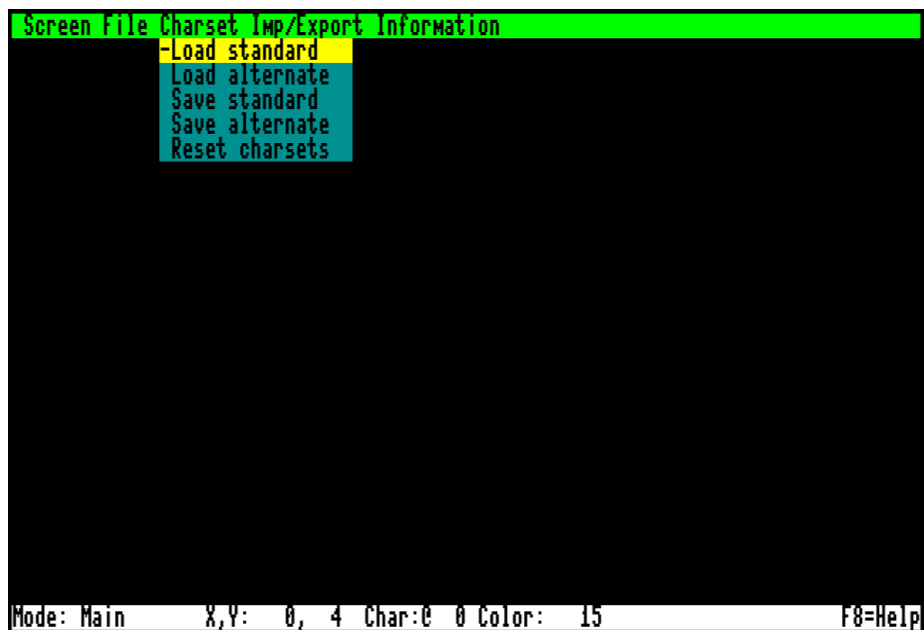
Figure 17: Charset menu
