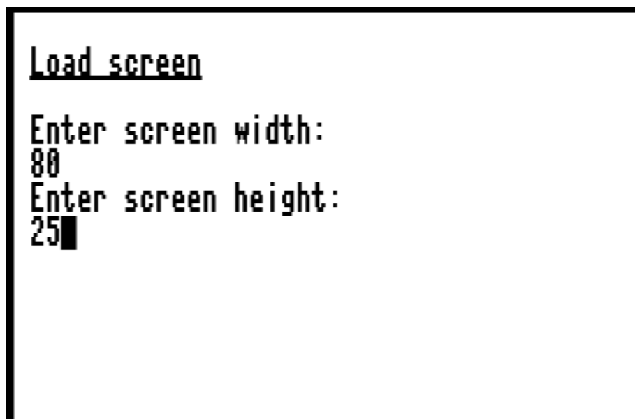
Figure 15: Load screen
