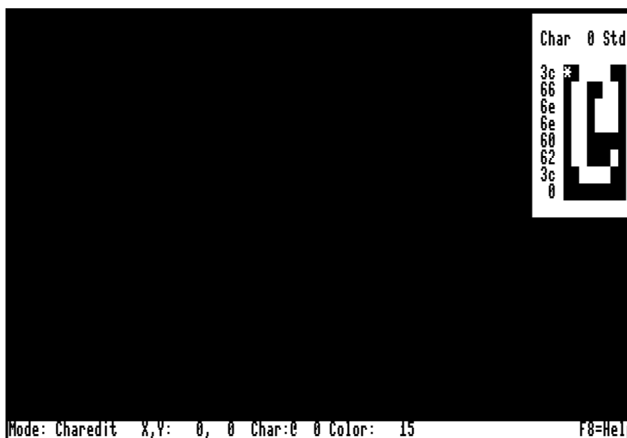
Figure 25: Character editor
