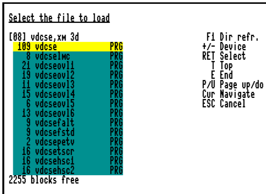
Figure 14: File picker
