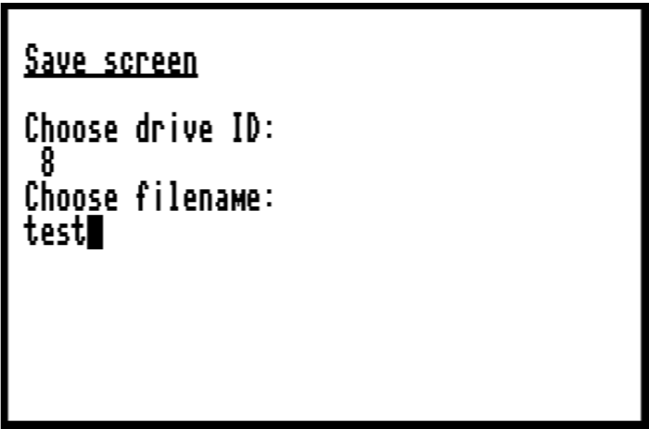
Figure 13: Choose filename
