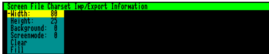
Figure 5: Screen menu
