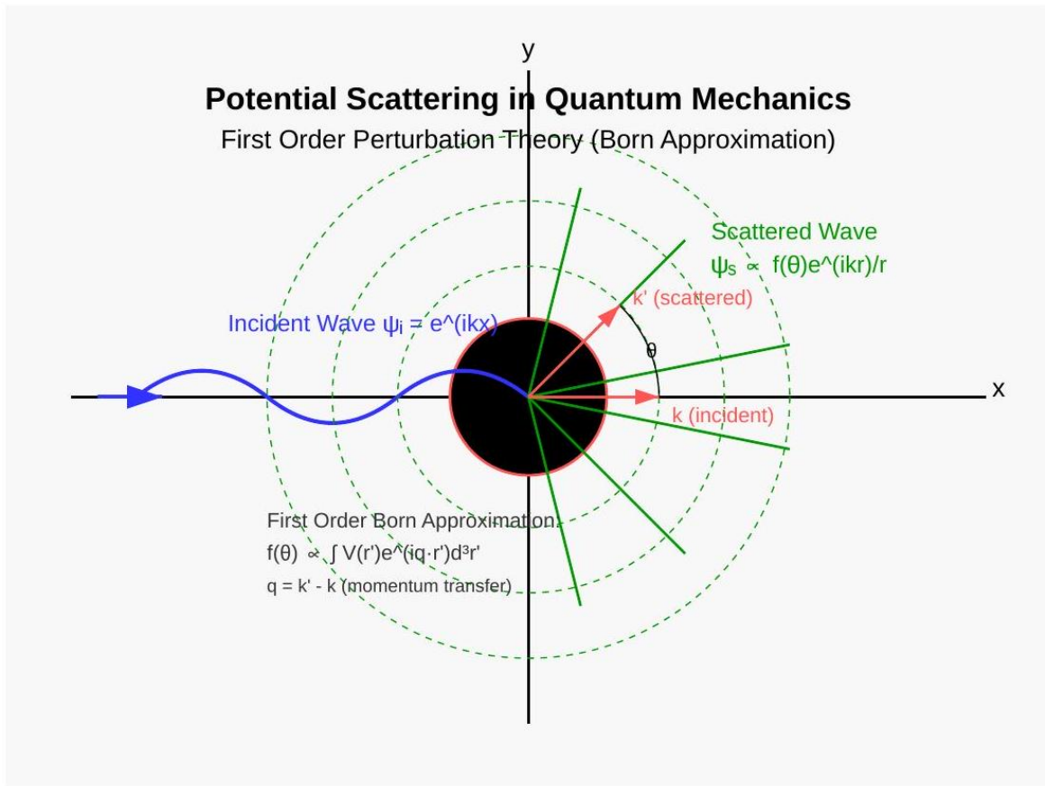
Figure 10.1: Potentialstreuung Illustration
