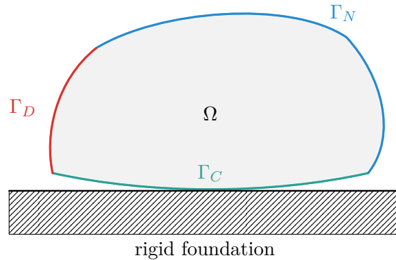
Figure 1: 2D Setup for Signorini's Problem.
