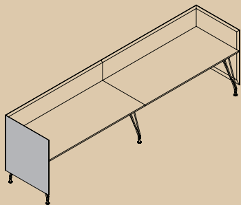
L x W 320x80 / 360x80 / 420x80 H 105 Panel suspendido / Suspended Panel Madera / Lacado / Melamina / Cristal Wood / Lacquered / Melamine / Glass
