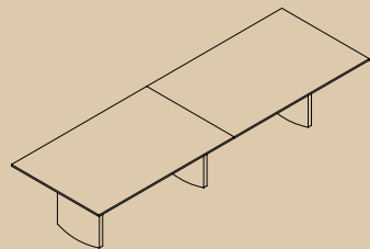
L x W 360x100 / 400x120 / 420x120 / 440x120 H 73 Madera / Lacado Wood / Lacquered
