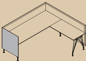
L x W 200x80-180 / 220x80-180 / 240x80-180 H 105 Panel suspendido / Suspended Panel Madera / Lacado / Melamina / Cristal Wood / Lacquered / Melamine / Glass
