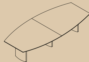
L x W 360x100 / 400x120 / 420x120 / 440x120 H 73 Madera / Lacado Wood / Lacquered
