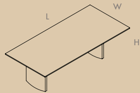
L x W 200x100 / 220x120 / 240x120 / 260x120 H 73 Madera / Lacado Wood / Lacquered
