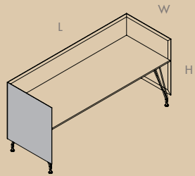
L x W 200x80 / 220x80 / 240x80 H 105 Panel suspendido / Suspended Panel Madera / Lacado / Melamina / Cristal Wood / Lacquered / Melamine / Glass
