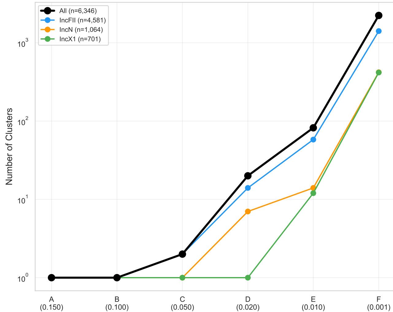
A. Clustering Resolution vs. Threshold
