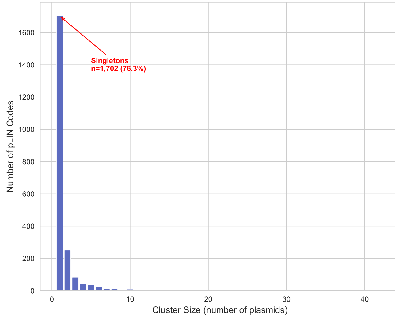
B. Strain-Level Cluster Size Distribution (Bin F, d \leq 0.001 )
