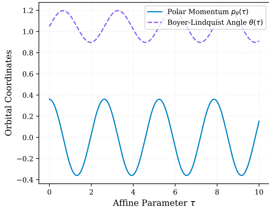
(a) Symplectic Kerr Geodesic Flow ( |\Delta Q|/Q_0 = 3.64 \times 10^{-13} )
