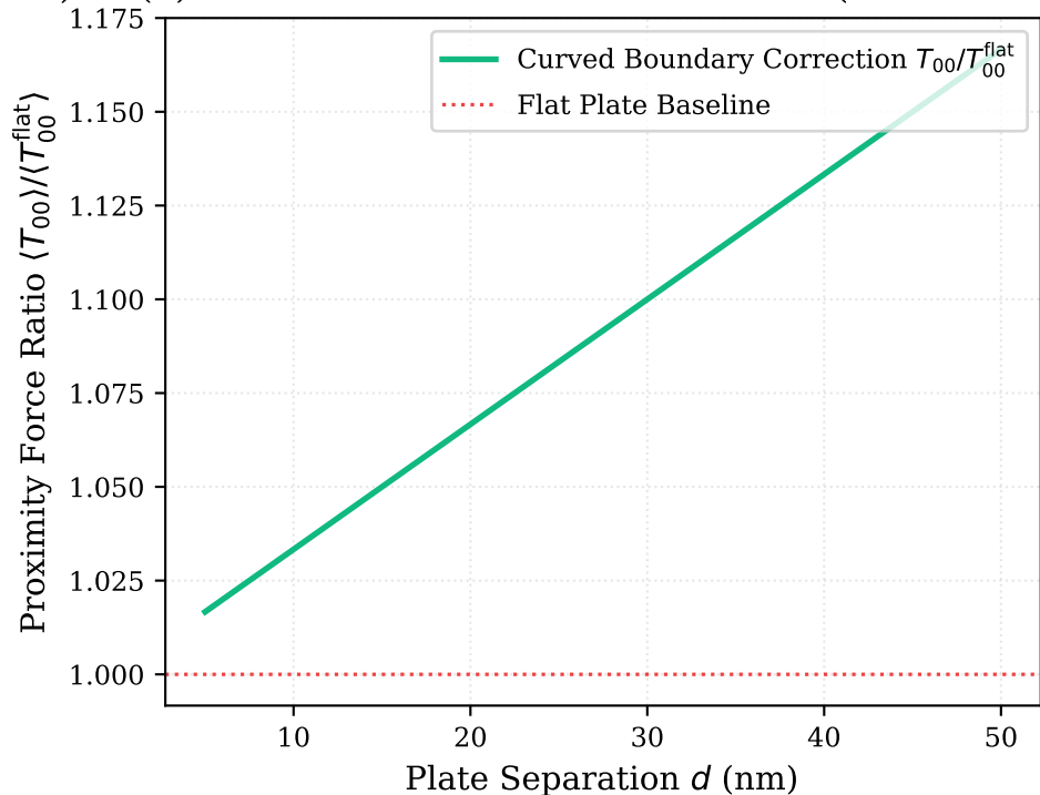
(b) Casimir Vacuum Stress Correction ( R = 100 nm)
