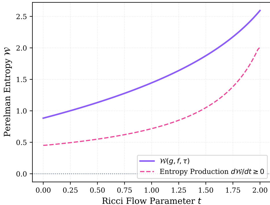
(b) Monotonic Ricci Flow Entropy ( d^2 = 0 Attested)
