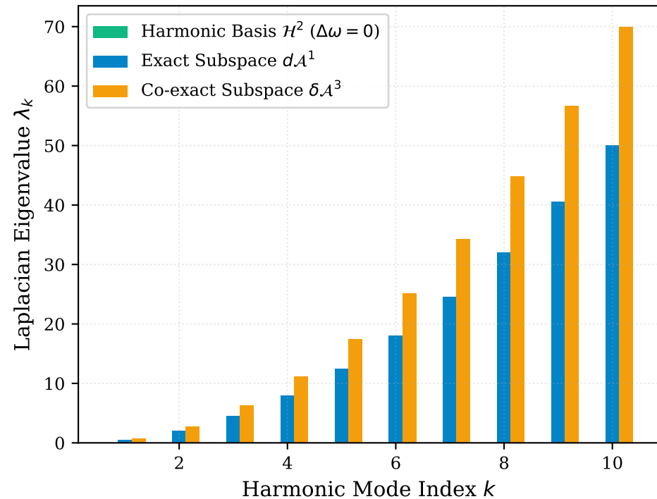
(a) Hodge Decomposition Spectrum ( \Delta = d\delta + \delta d )
