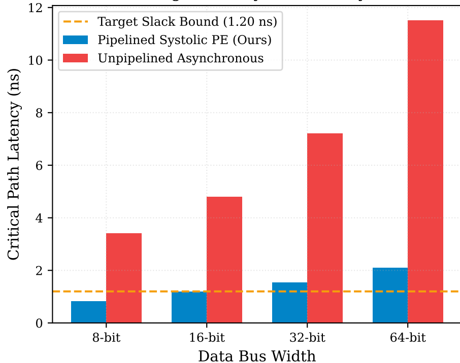
(a) RTL Timing Slack: Synthesized Systolic Core
