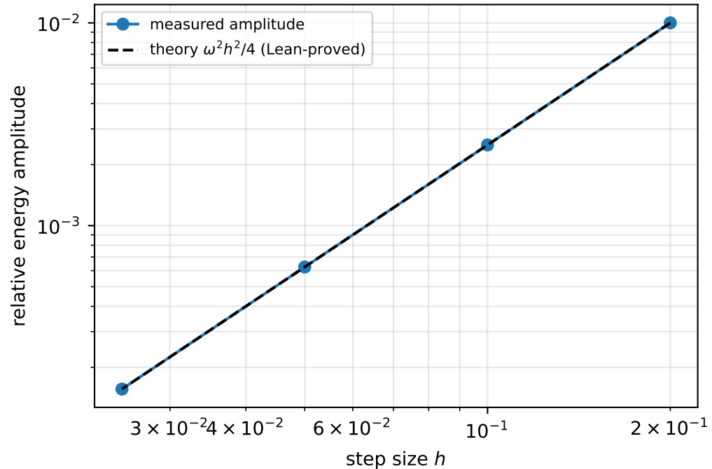
O(h^2) scaling
