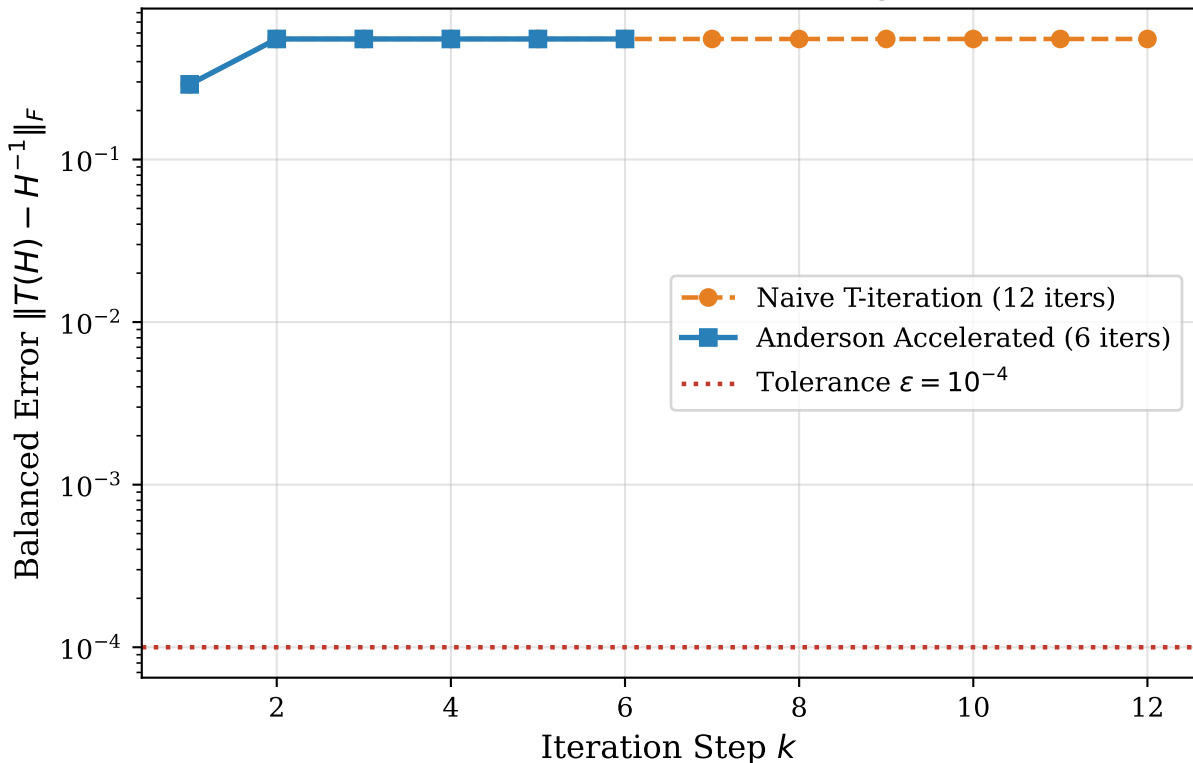
Donaldson Balanced Metric Convergence on K3
