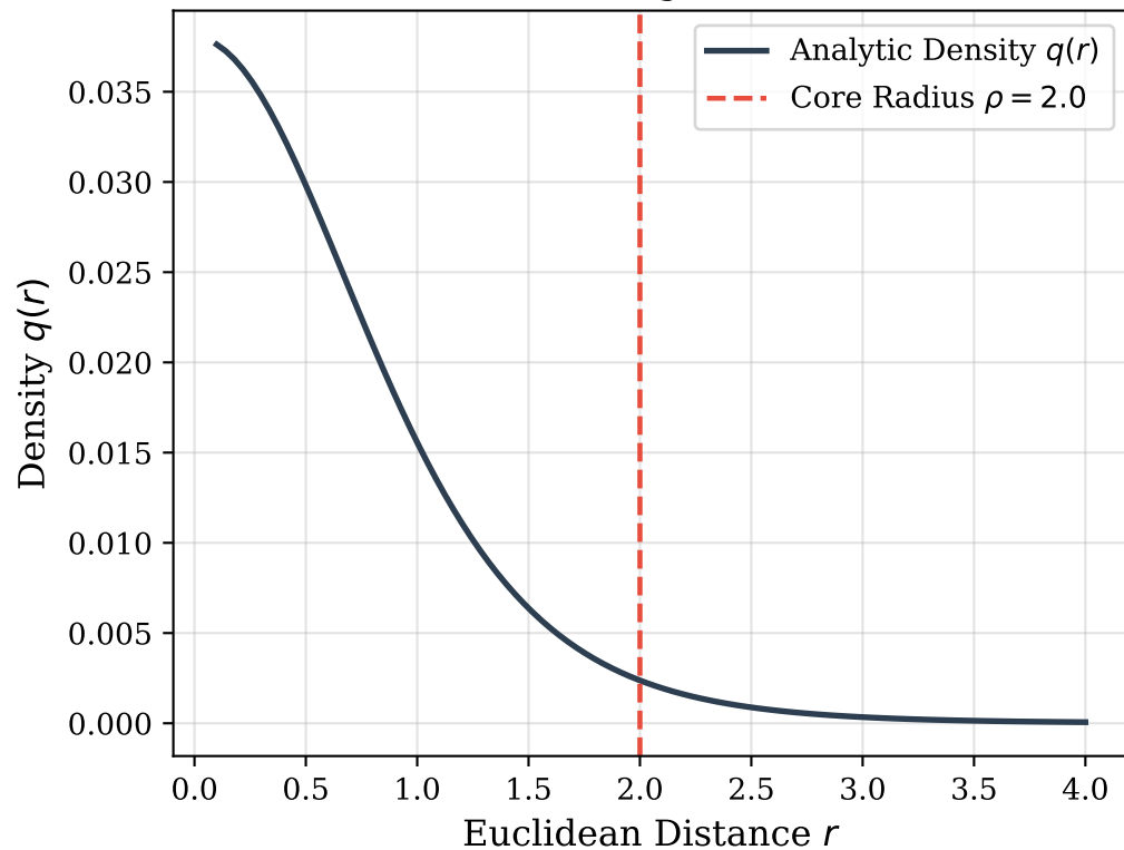
Quantized Charge: c_2 = 0.8563
