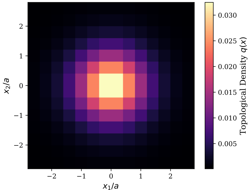
4D Lattice BPST Instanton Slice
