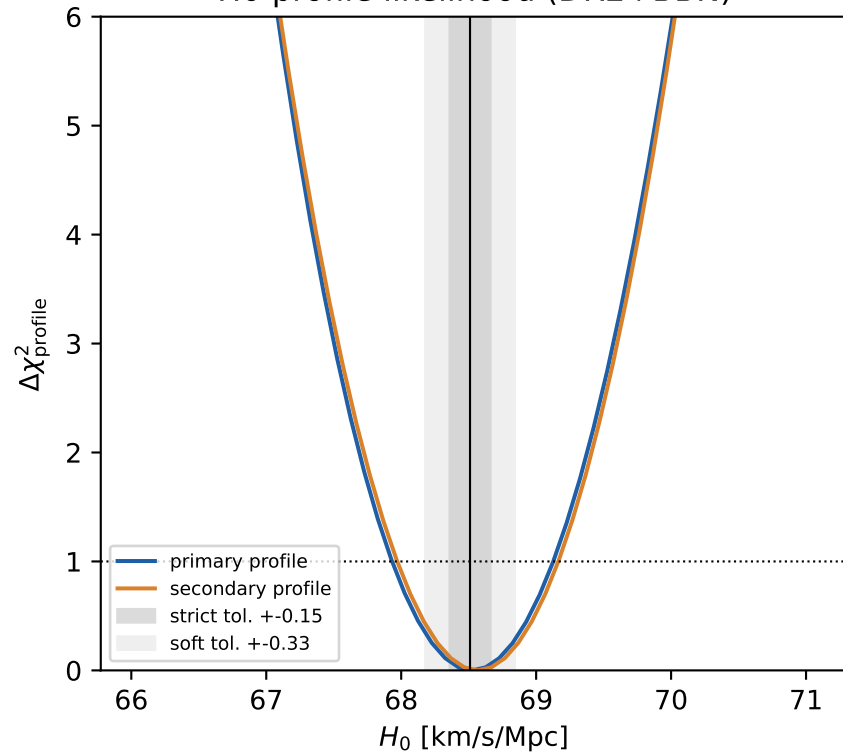
H0 profile likelihood (DR2+BBN)
