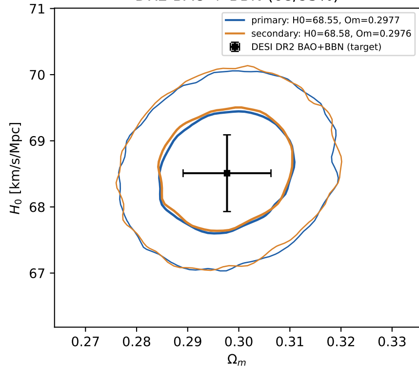
DR2 BAO + BBN (68/95%)
