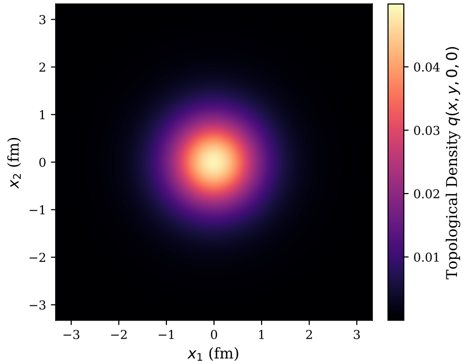
(b) Lattice Instanton Density ( Q_{\text{top}} = 0.9455 )
