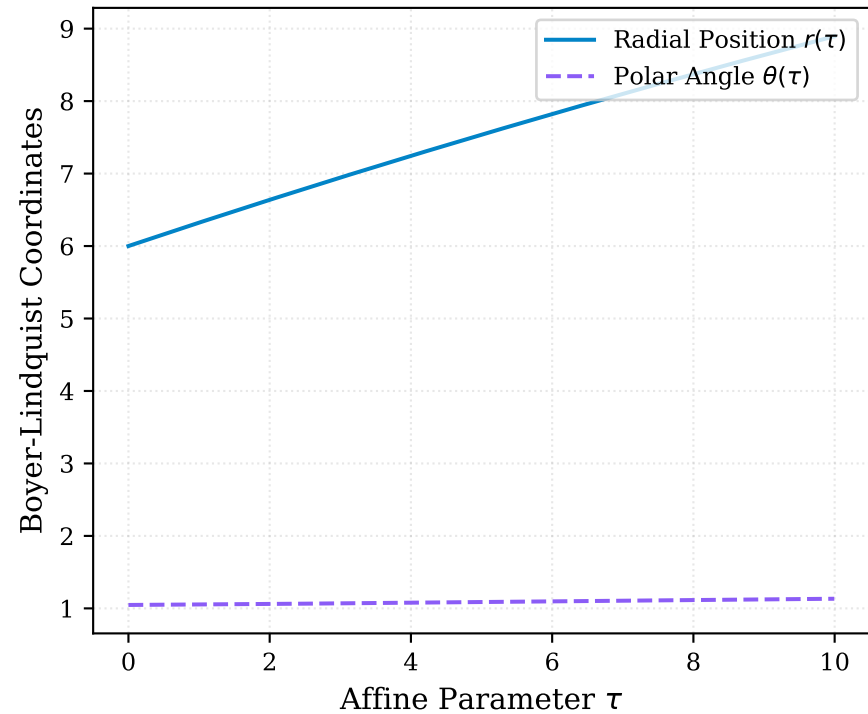
(a) Kerr Geodesic Orbit ( \text{Var}(r)=0.70 , \varepsilon_Q=3.3\text{e-}11 )
