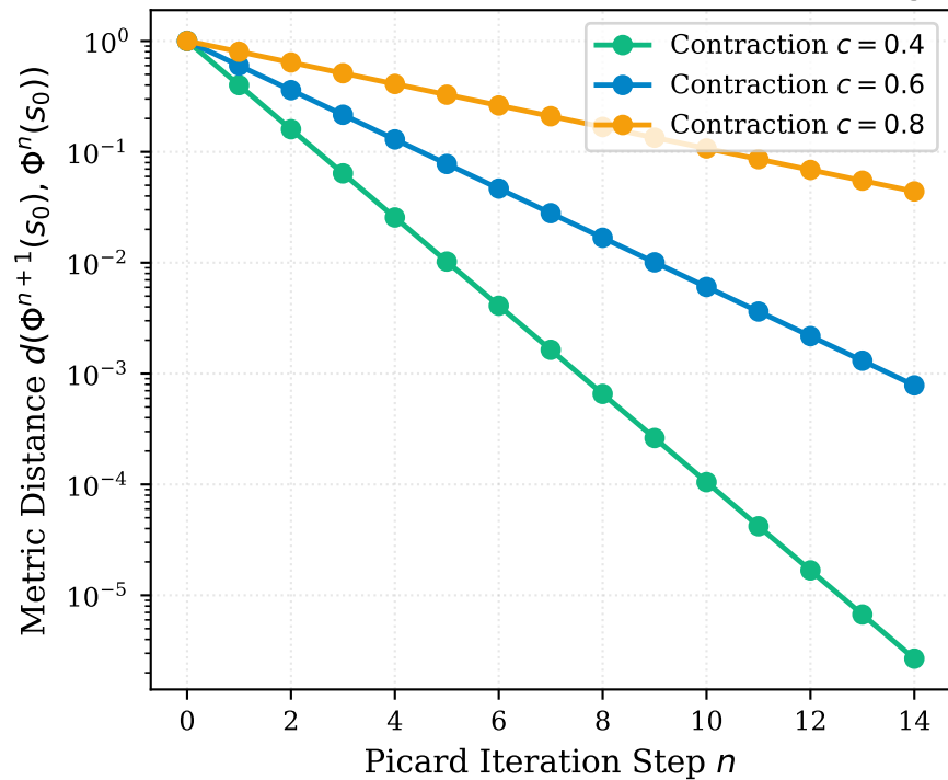
(b) Lean 4 Proven Banach Fixed-Point Convergence
