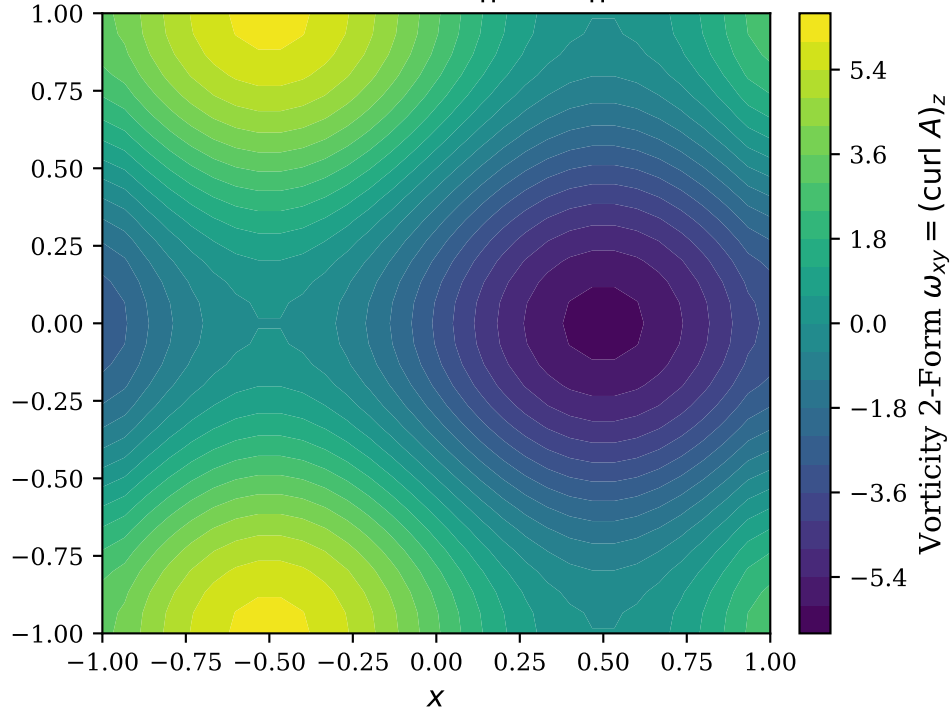
(a) Discrete Exterior 2-Form ( \|d(dA)\|_\infty = 1.15 \times 10^{-14} )
