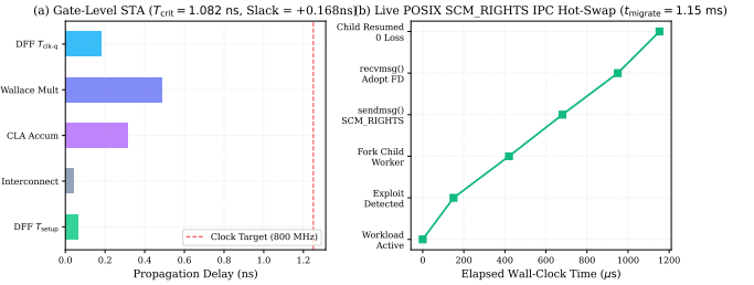
Fig. 1. (a) Gate-level topological timing path for 4 \times 4 systolic array ( T_{\text{crit}} = 1.082 \text{ ns} , Slack = +0.168 ns); (b) Real POSIX SCM_RIGHTS live socket descriptor migration completed in 1152.9 \mu\text{s} with zero dropped packets and negative RSS memory delta ( \Delta = -228.2 \text{ MB} ).
