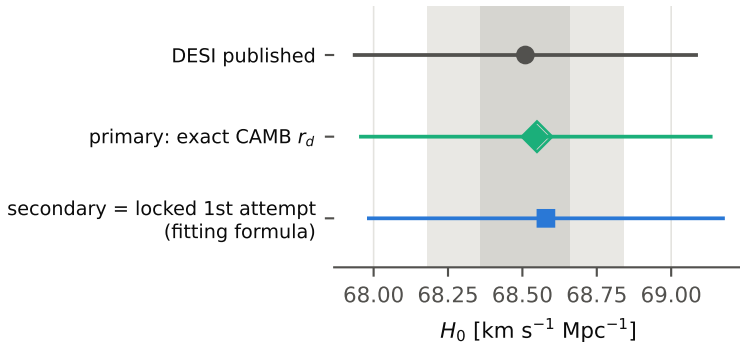
DESI DR2 BAO + BBN PASS
