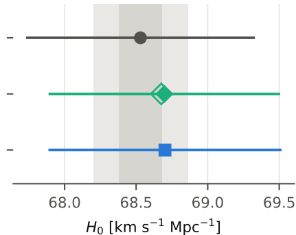
DESI DR1 BAO + BBN PARTIAL (recorded run) / PASS (re-run)
