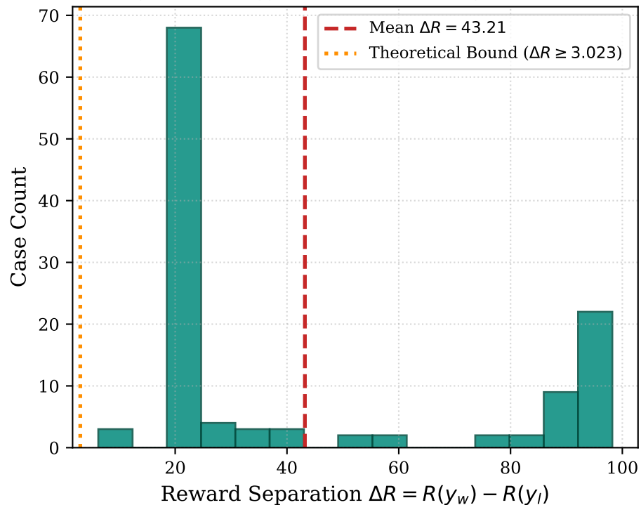
(a) Physical Energy DPO Reward Margin Distribution
