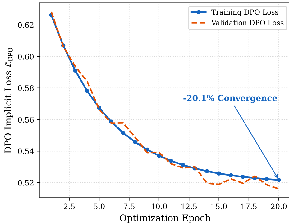
(b) LoRA Fine-Tuning Convergence (-20.1% Loss)
