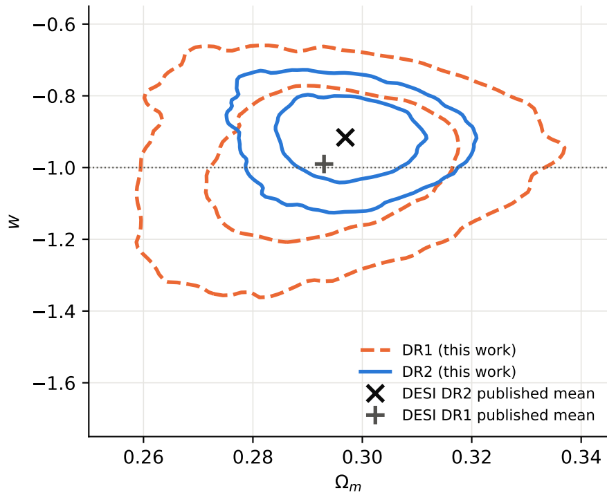
Flat w CDM, BAO only (68%, 95%)
