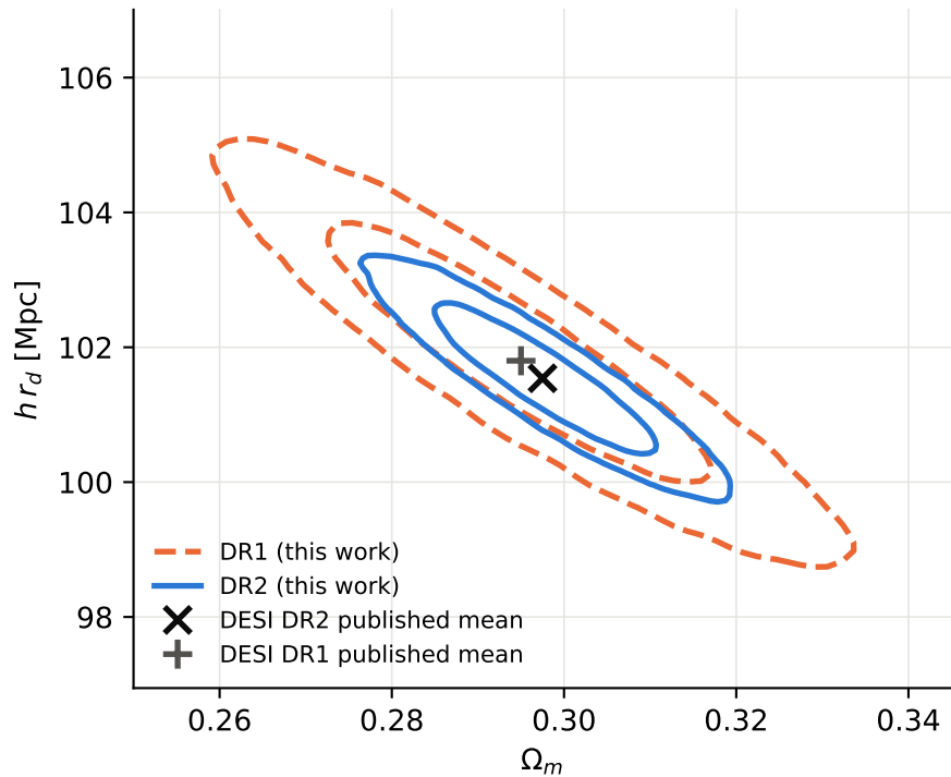
Flat \Lambda CDM, BAO only (68%, 95%)
