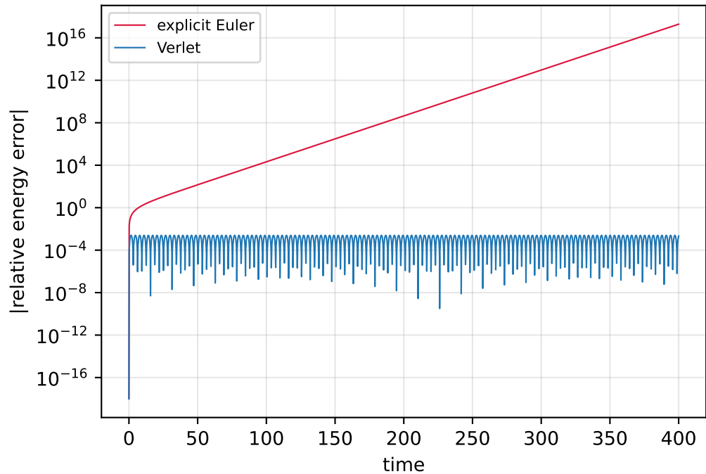
Secular drift: Euler diverges, Verlet does not
