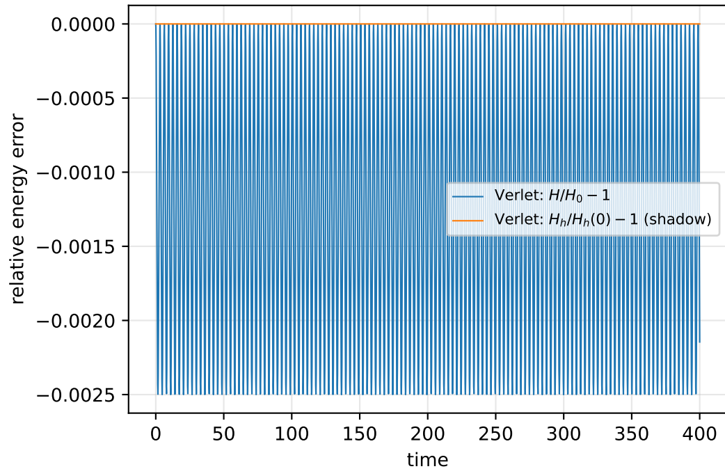
Störmer-Verlet, h = 0.1 : bounded, non-drifting
