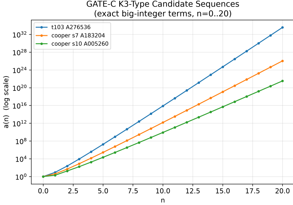
Figure 7: Exact big-integer terms of the three GATE-C K3-type candidate sequences, n = 0..20 (log scale).
