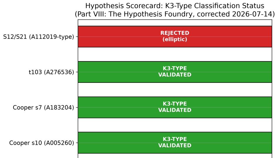
Figure 11: Summary scorecard: K3-type classification status per candidate.
