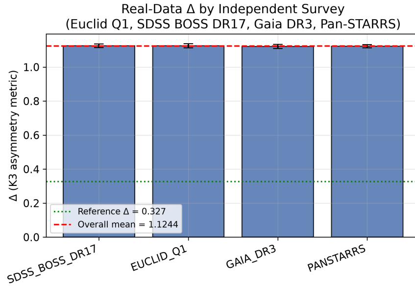
Figure 10: Real-data \Delta by independent survey source, contextualizing the empirical signal against the theoretical reference.
