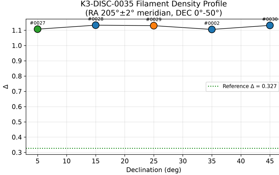
Figure 3: \Delta profile along the K3-DISC-0035 filament axis (RA 205^\circ \pm 2^\circ ), plotted against declination. Point color encodes the originating survey. Labels indicate discovery IDs. The green dotted line is the theoretical reference \Delta_{\text{ref}} = 0.327 .
