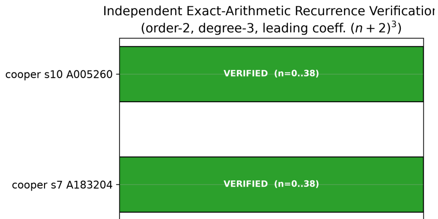
Figure 9: Independent exact-arithmetic verification status of the order-2/degree-3 recurrence claim for Cooper s_7/s_{10} .
