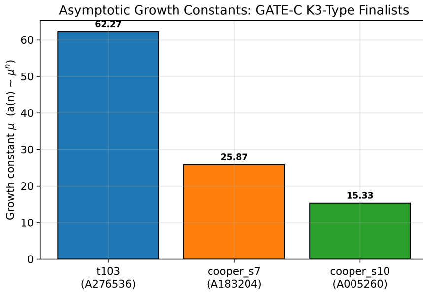
Figure 8: Estimated asymptotic growth constants \mu for the three finalists.
