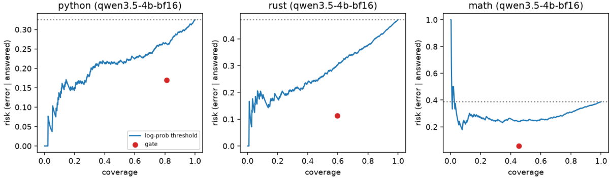
Figure 4: Qwen3.5-4B (bf16, TPU), full E set, exploratory; revision 3.5.0, with the program-of-thought math gate. Blue: risk-coverage curve of a raw log-prob threshold (risk = error rate among answered tasks ). Red dot: the executed gate, whose risk is one minus its precision. Dotted line: error rate when every task is answered. Math now has a gate point. The left end of each curve rests on very few tasks.
