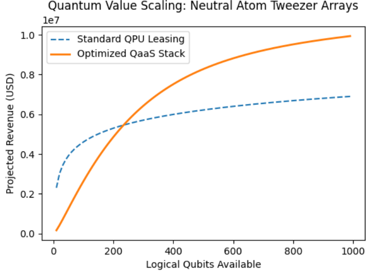
Figure 4: Quantum Value Scaling Simulation
