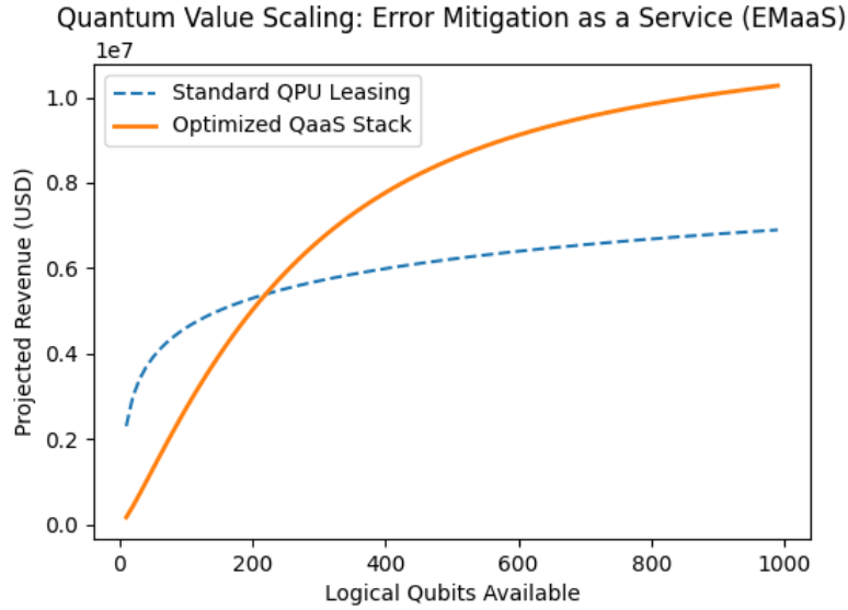
Figure 3: Quantum Value Scaling Simulation
