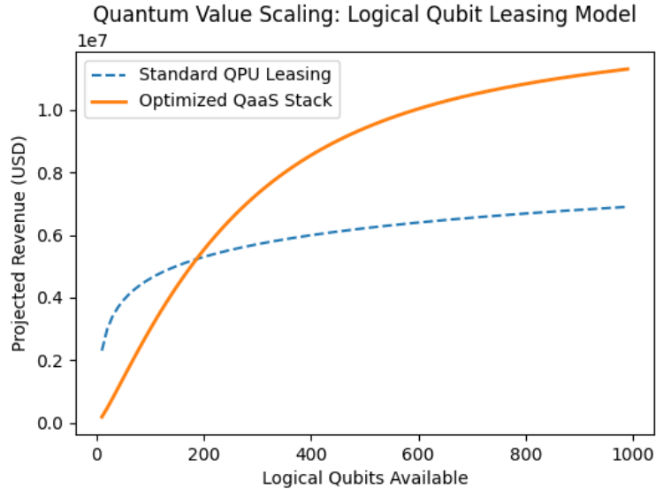
Figure 1: Quantum Value Scaling Simulation
