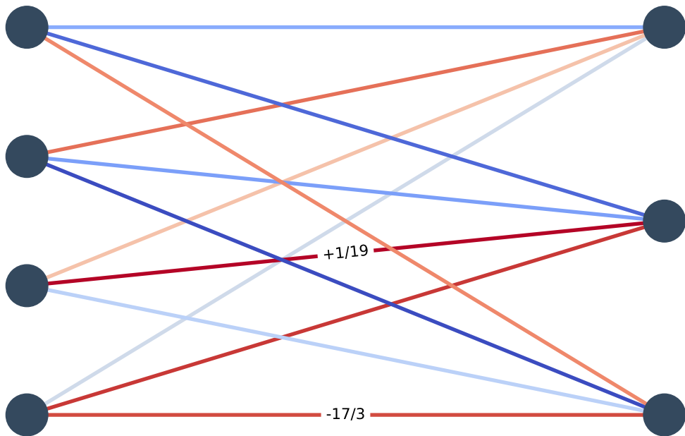
Fractional Charging Matrix \omega(u, v) on K_{4,3}
