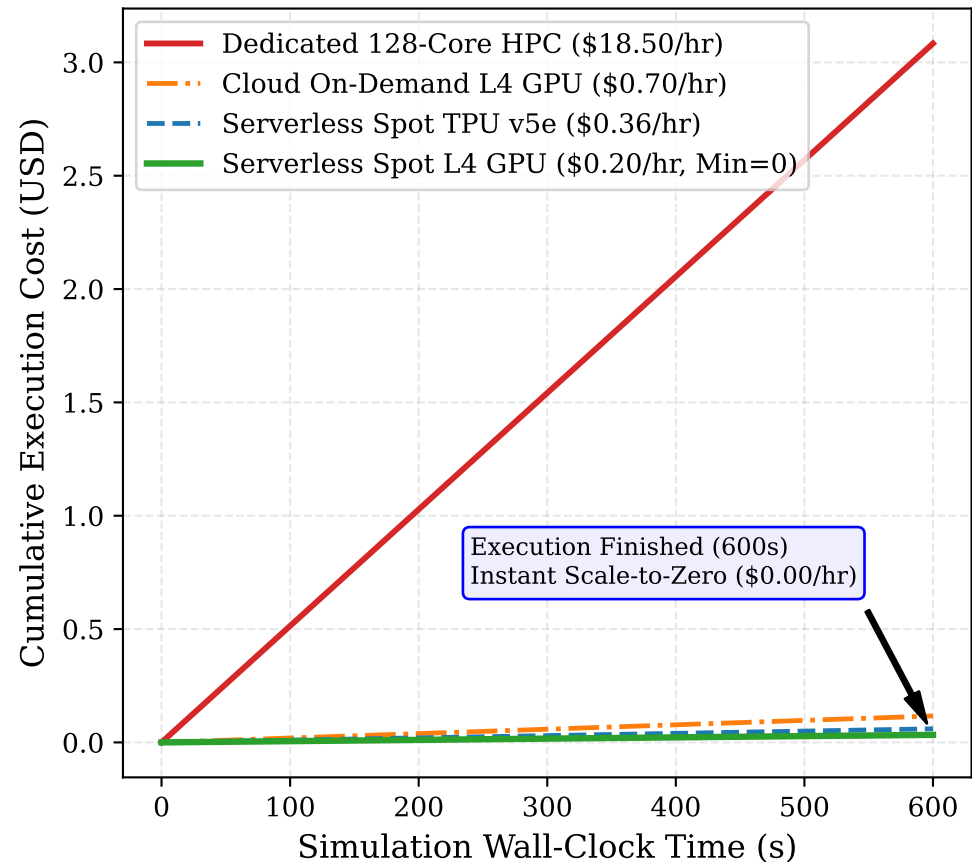
(a) Serverless Spot Cost vs Dedicated HPC
