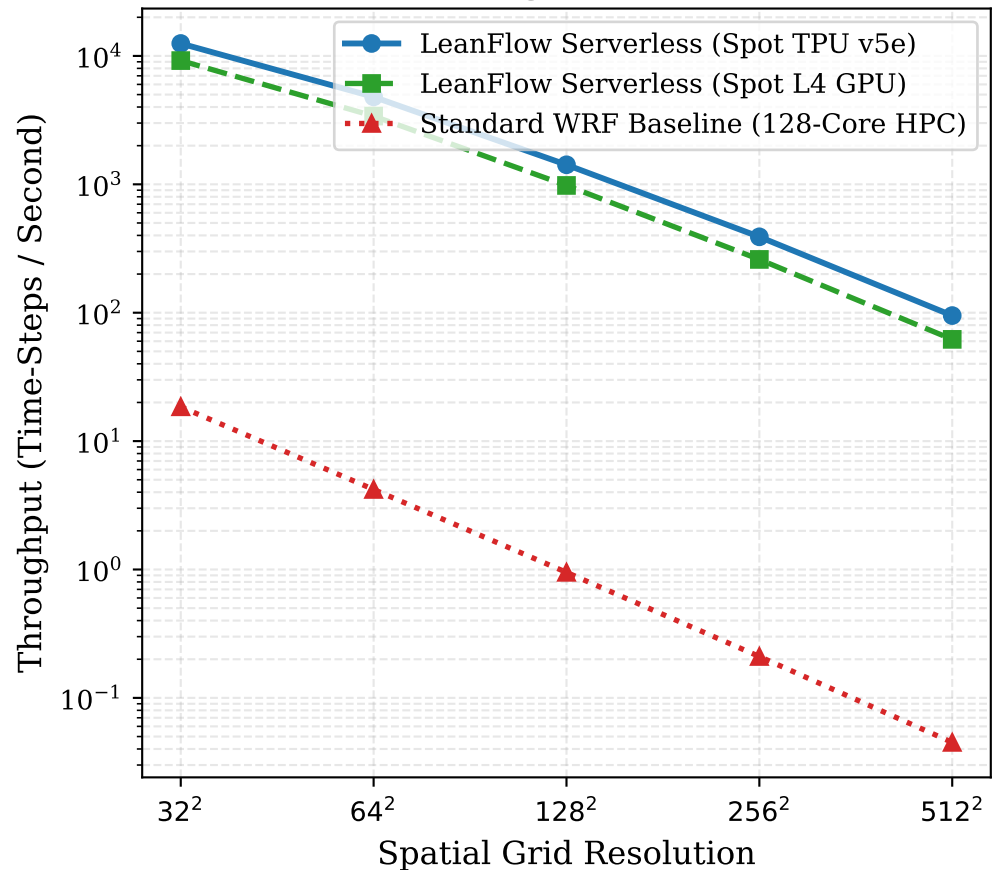
(b) Compute Scaling & Resolution Speedup
