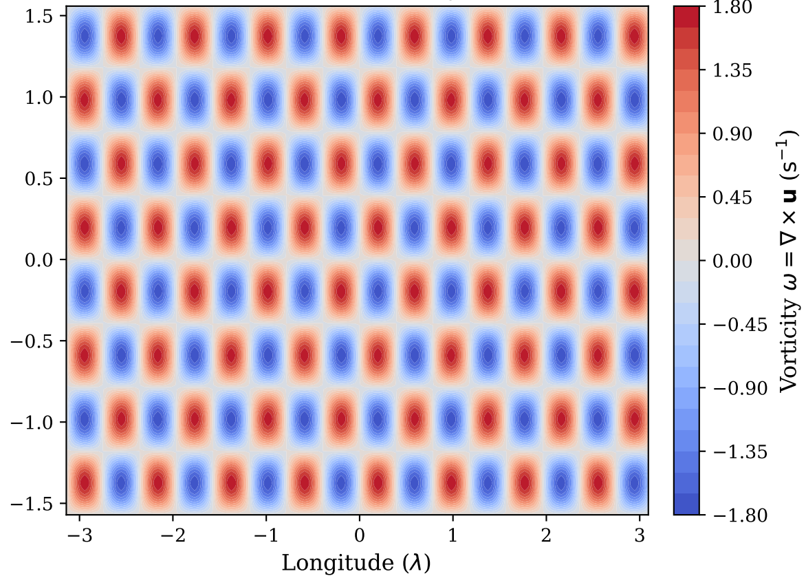
(b) Micro-Turbulent Vorticity Cascade \omega(\mathbf{x})
