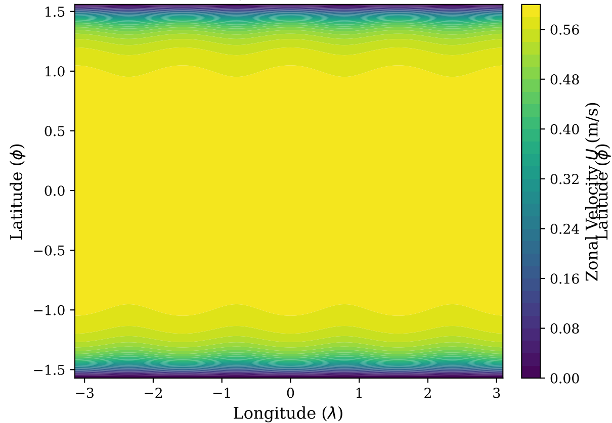
(a) Planetary Jet Stream Field U(\mathbf{x})
