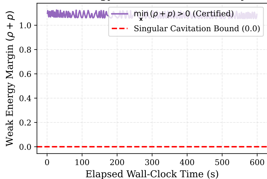
(c) Weak Energy Condition via F-Theory \tau_{\text{im}} > 0
