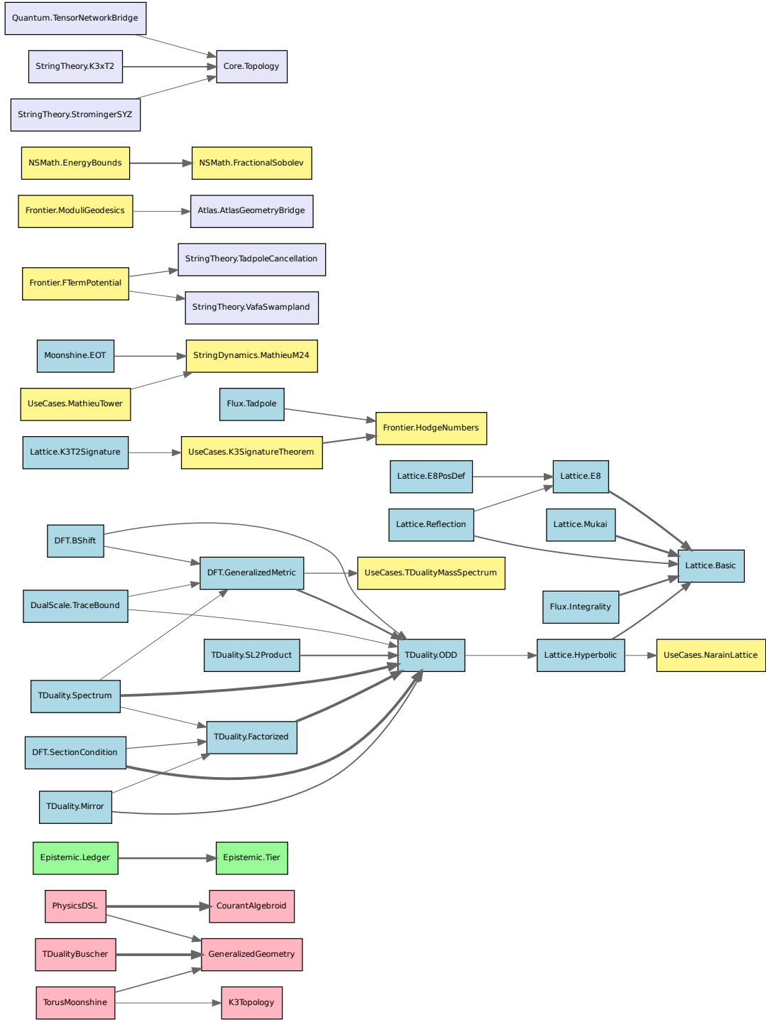
Figure 36.1: Module-level dependency graph extracted from the kernel: 44 modules, 42 edges. Colours mark libraries (blue: DualScaleStream2 ; yellow: StringTheoryFormalization ; pink: DoubleFieldTheory ; green: DualScaleM24Formalization ; lavender: StringTheoryFoundation ). An arrow from M to M' means a declaration of M uses a declaration of M' . Generated by tools/theorem_atlas.py from .leancache/depgraph.jsonl ; the source PDF is legible at higher magnification.
