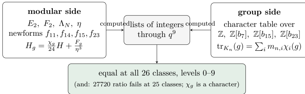
Figure 39.1: The two routes of this chapter. Neither side is copied from the other: the left side is computed from modular forms, the right side from a guarded character table, and the comparison is made on finite lists of integers.
