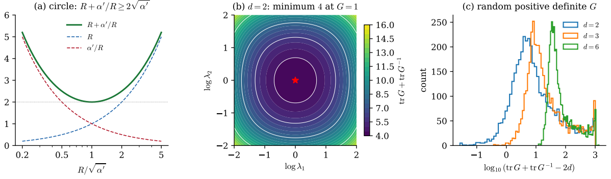
Figure 2: The dual-scale bound. (a) On a circle the effective scale R + \alpha'/R is minimized at the self-dual radius. (b) For d = 2 and positive-definite G with eigenvalues \lambda_{1,2} , \text{tr } G + \text{tr } G^{-1} = \sum_i (\lambda_i + \lambda_i^{-1}) has its minimum 2d = 4 at G = 1 . (c) Excess over 2d for 4000 random positive definite matrices in each dimension: never negative, as the Lean theorem dualScale_ge guarantees. The plot illustrates the theorem; it proves nothing. Computed figure; data: Lean dualScale_circle , circle_effective_scale_ge_two , dualScale_ge (TraceBound.lean).
