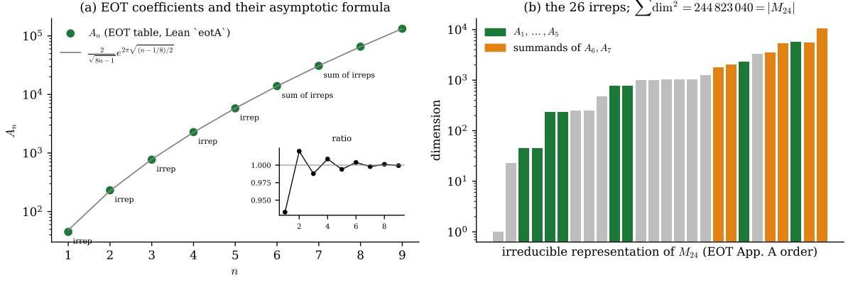
Figure 3: (a) The coefficients A_n of the K3 elliptic genus (EOT eq. 1.12, the Lean table eotA ) against the asymptotic formula EOT eq. (1.13); the inset shows the ratio. A_1, \dots, A_5 are dimensions of irreducible representations of M_{24} ; A_6 and A_7 are sums of them. (b) The 26 irreducible dimensions of M_{24} from the Lean table M24RepDim ; the sum of their squares equals the group order ( M24RepDim_sum_sq ), the check that caught an earlier wrong table. Computed figure; data: EOT eqs. (1.12)–(1.15), ll. 200–232 (formula read from the PDF page, the .txt garbles it); App. A (A.3).
