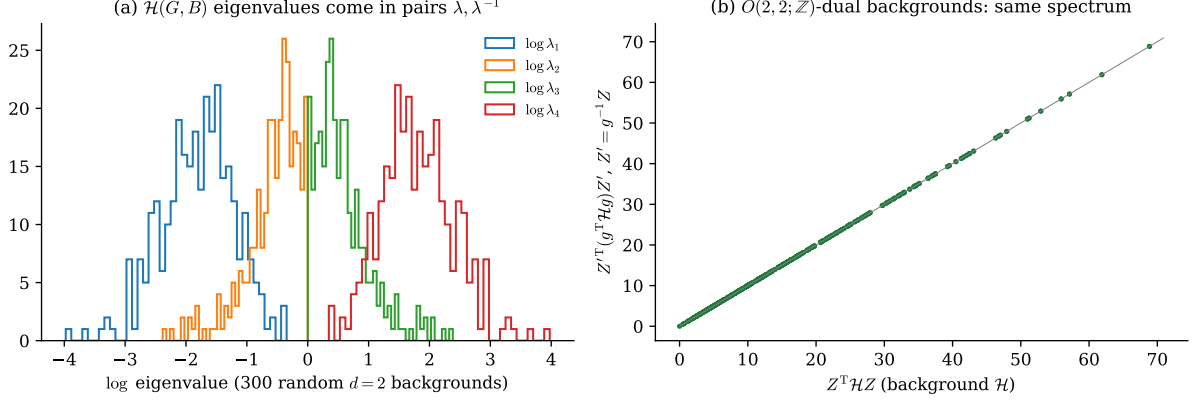
Figure 5: (a) Logarithms of the four eigenvalues of the generalized metric \mathcal{H}(G, B) for 300 random backgrounds on T^2 : they are symmetric about 0, because (\eta\mathcal{H})^2 = 1 ( etaR_genMetric_sq ) forces eigenvalues in pairs \lambda, \lambda^{-1} . (b) For g = \Theta \cdot A \cdot (\text{factorized duality}) \cdot \Theta' \in O(2, 2; \mathbb{Z}) , the mass form of every charge Z in background \mathcal{H} equals that of g^{-1}Z in the dual background g^T \mathcal{H} g : the points lie on the diagonal ( spectrum_equivalence, massForm_covariant ). Computed figure; data: Lean genMetric (GeneralizedMetric.lean), thetaShift, basisChange, factorized; HHZ §2.
