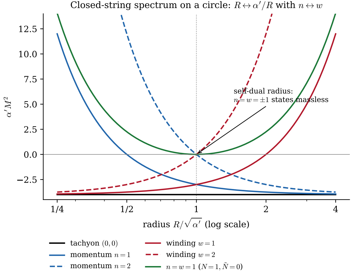
Figure 4: Lowest mass levels of the closed bosonic string on a circle of radius R as a function of \log R , with the lowest oscillator levels allowed by level matching N - \tilde{N} = nw . Momentum and winding curves are mirror images under R \mapsto \alpha'/R ; at the self-dual radius the n = w = \pm 1 states become massless (enhanced gauge symmetry). Computed figure; data: Tong §8.2, ll. 11351–11470; Lean leftMomentum, rightMomentum (units \alpha' = 1 ).
